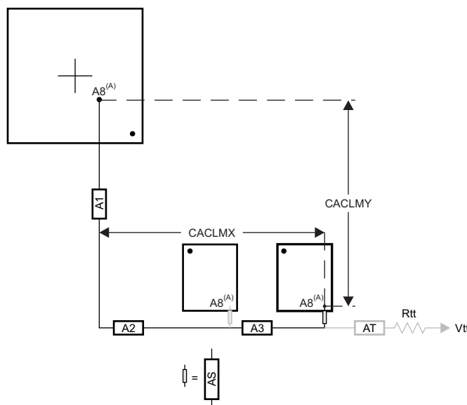
FIG 8-26. CACLM for Four Address Loads on One Side of PCB
