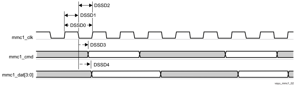
図 7-61. MMC/SD/SDIO in - Default Speed - Transmitter Mode
