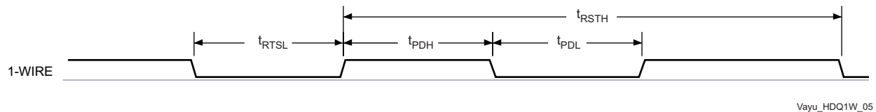
图 7-29. 1-Wire—Break (Reset)
