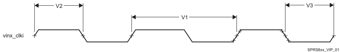
図 7-4. Video Input Ports Clock Signal
