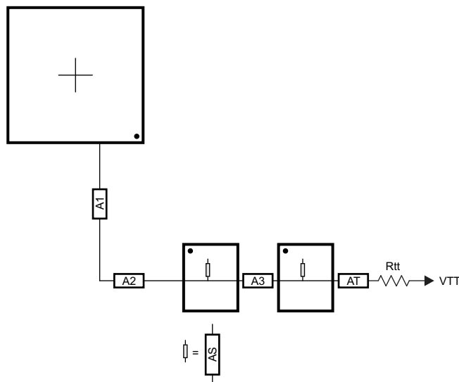
FIG 8-15. ADDR_CTRL Routing for Two Single-Side DDR3 Devices
