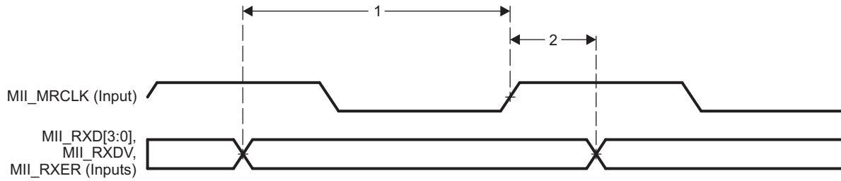
图 7-106. PRU-ICSS MII_RXD[3:0], MII_RXDV, and MII_RXER Timing
