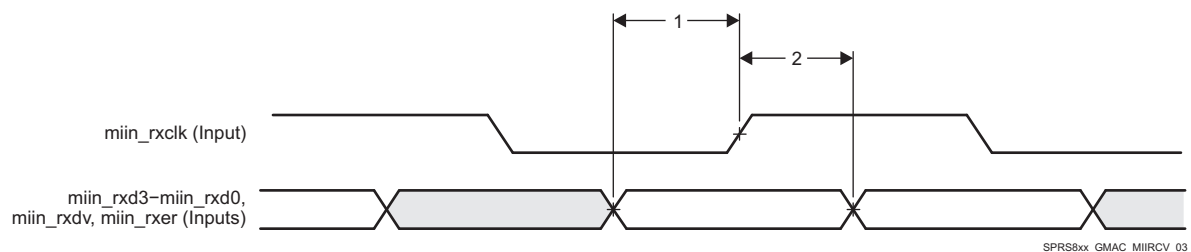
图 7-53. GMAC Receive Interface Timing MII operation
