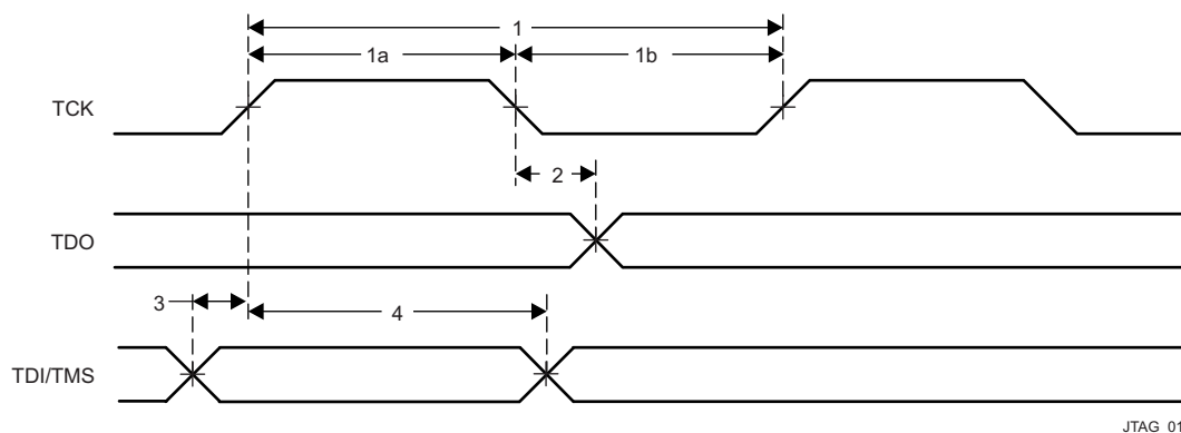
图 7-109. JTAG Timing
