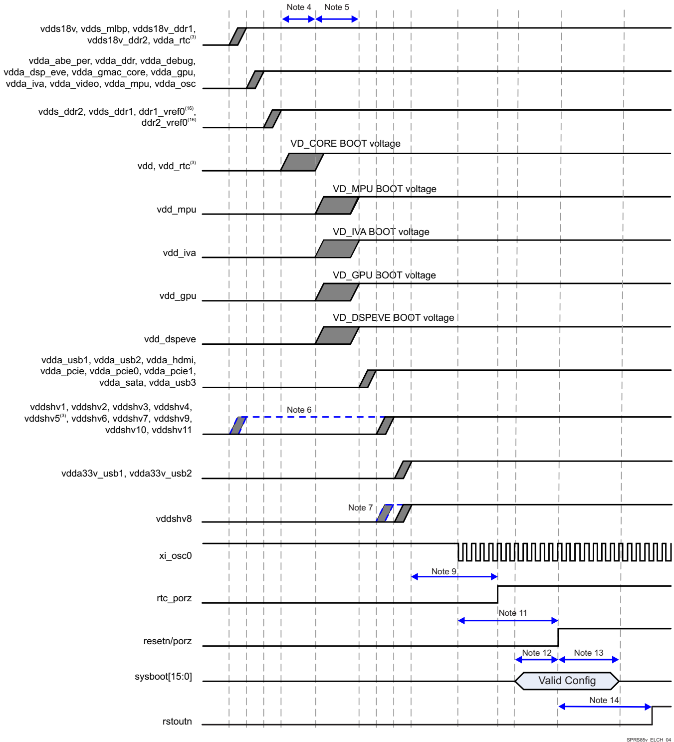
☒ 5-2. Power-Up Sequencing
