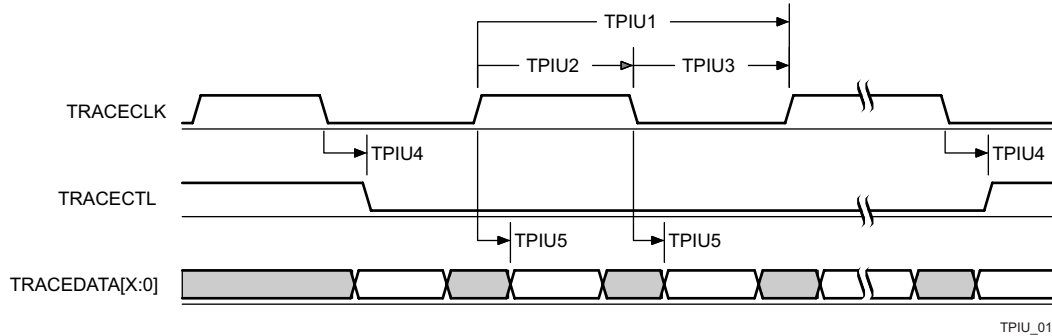
图 7-111. TPIU—PLL DDR Transmit Mode (1)
