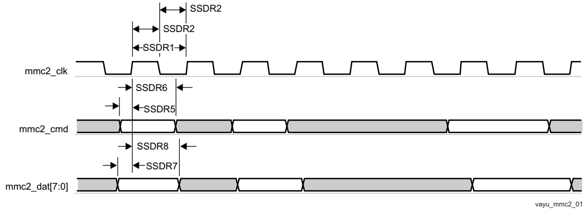
図 7-74. MMC/SD/SDIO in - Standard JC64 - Receiver Mode
