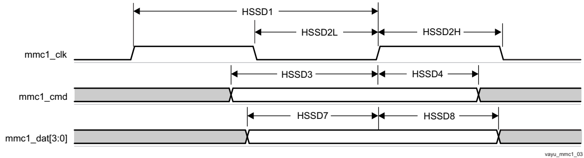
图 7-62. MMC/SD/SDIO in - High Speed - Receiver Mode
