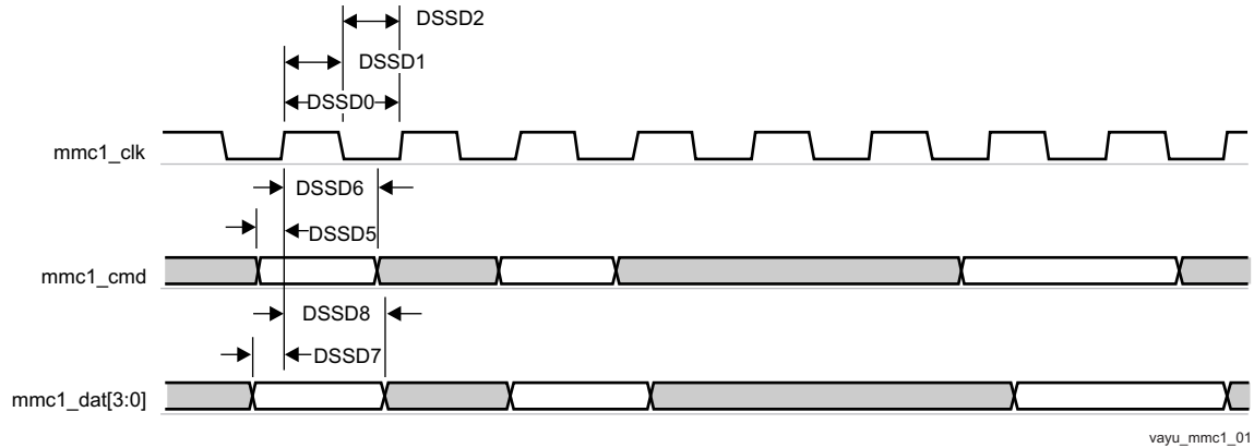
図 7-60. MMC/SD/SDIO in - Default Speed - Receiver Mode
