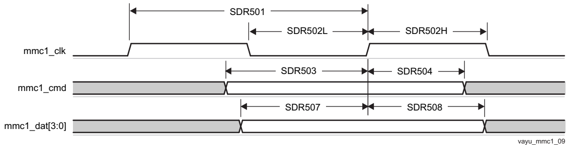
図 7-68. MMC/SD/SDIO in - High Speed SDR50 - Receiver Mode
