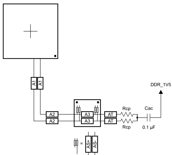
FIG 8-16. CK Routing for Two Mirrored DDR3 Devices
