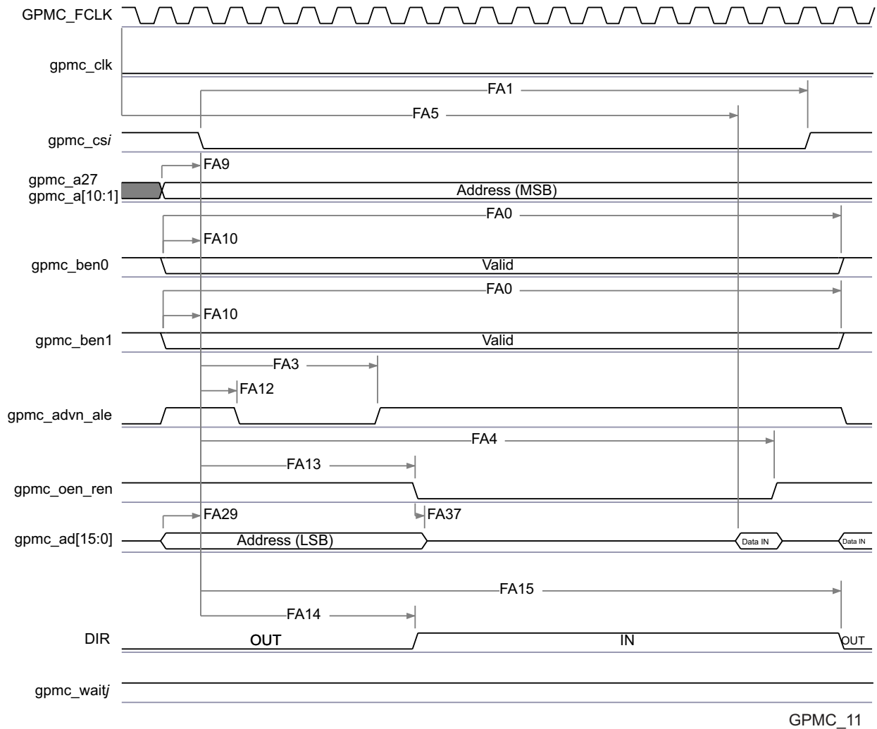
FIG 7-17. GPMC / Multiplexed NOR Flash - Asynchronous Read - Single Word Timing (1)(2)(3)
