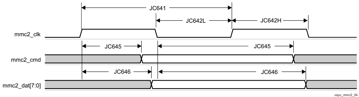
図 7-77. MMC/SD/SDIO in - High Speed JC64 - Transmitter Mode
