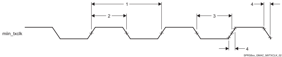
图 7-52. Clock Timing (GMAC Transmit) - MII operation
