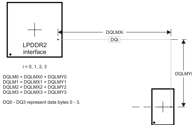
图 5-86. DQ[x] Routing
