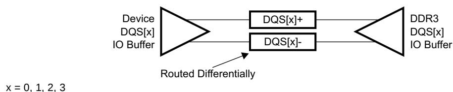
Figure 5-83. DQS[x] Topology
