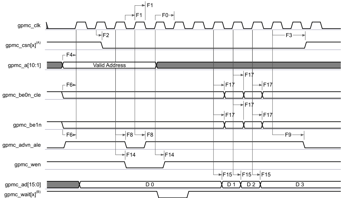
5-35. GPMC and NOR Flash—Synchronous Burst Write—(GpmcFCLKDivider > 0)
