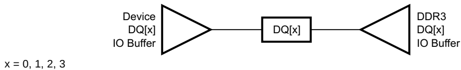
FIG 5-73. DQ[x] Topology
