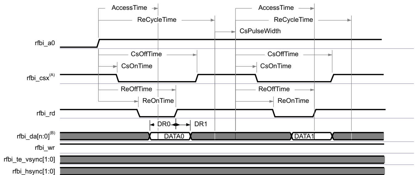
FIG 5-95. DSS—RFBI Mode—MIPI DBI 2.0—LCD Panel—Command / Data Write
