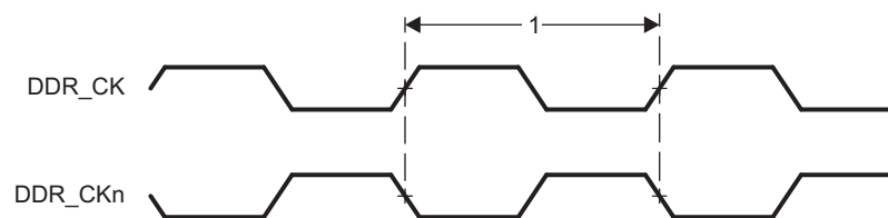
図 5-48. DDR3 Memory Interface Clock Timing
