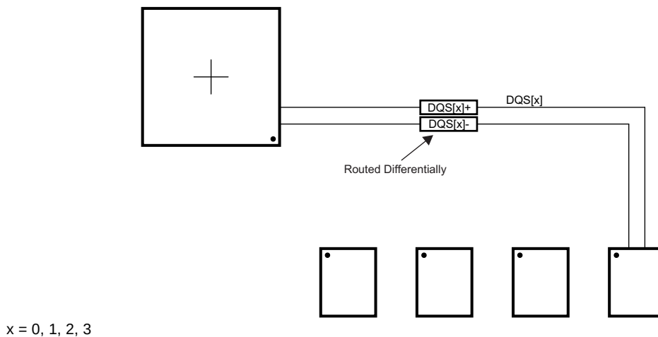
FIG 5-74. DQS[x] Routing With Any Number of Allowed DDR3 Devices
