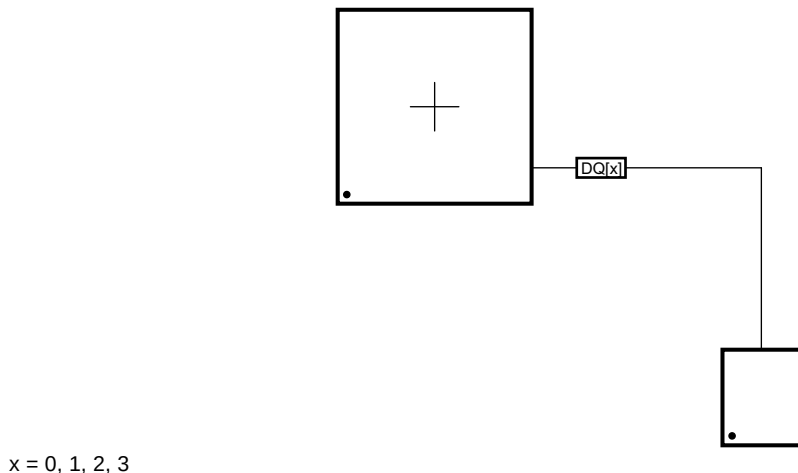
图 5-86. DQ[x] Routing
