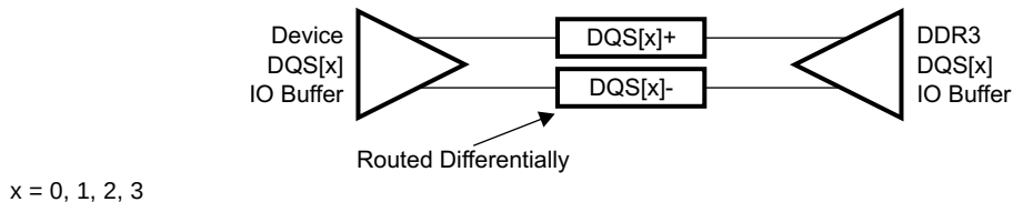
FIG 5-72. DQS[x] Topology
