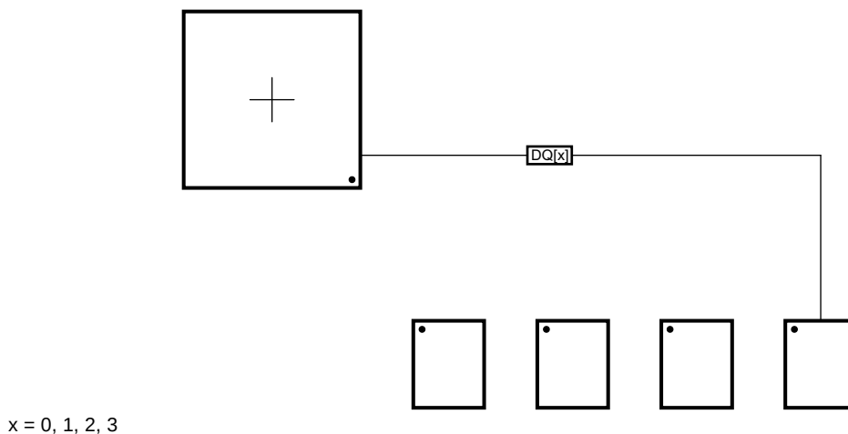
FIG 5-75. DQ[x] Routing With Any Number of Allowed DDR3 Devices
