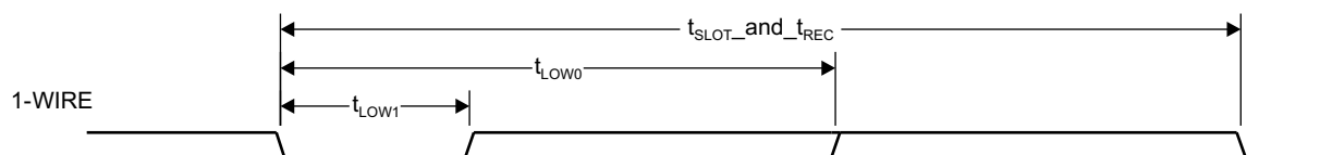
✎ 5-118. 1-Wire Write Bit Timing (Command/Address or Data)
