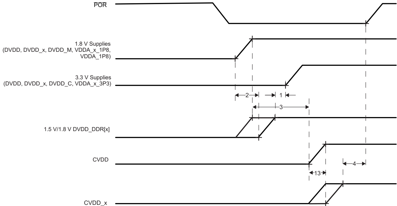
Figure 8-1. Power-Up Sequence
