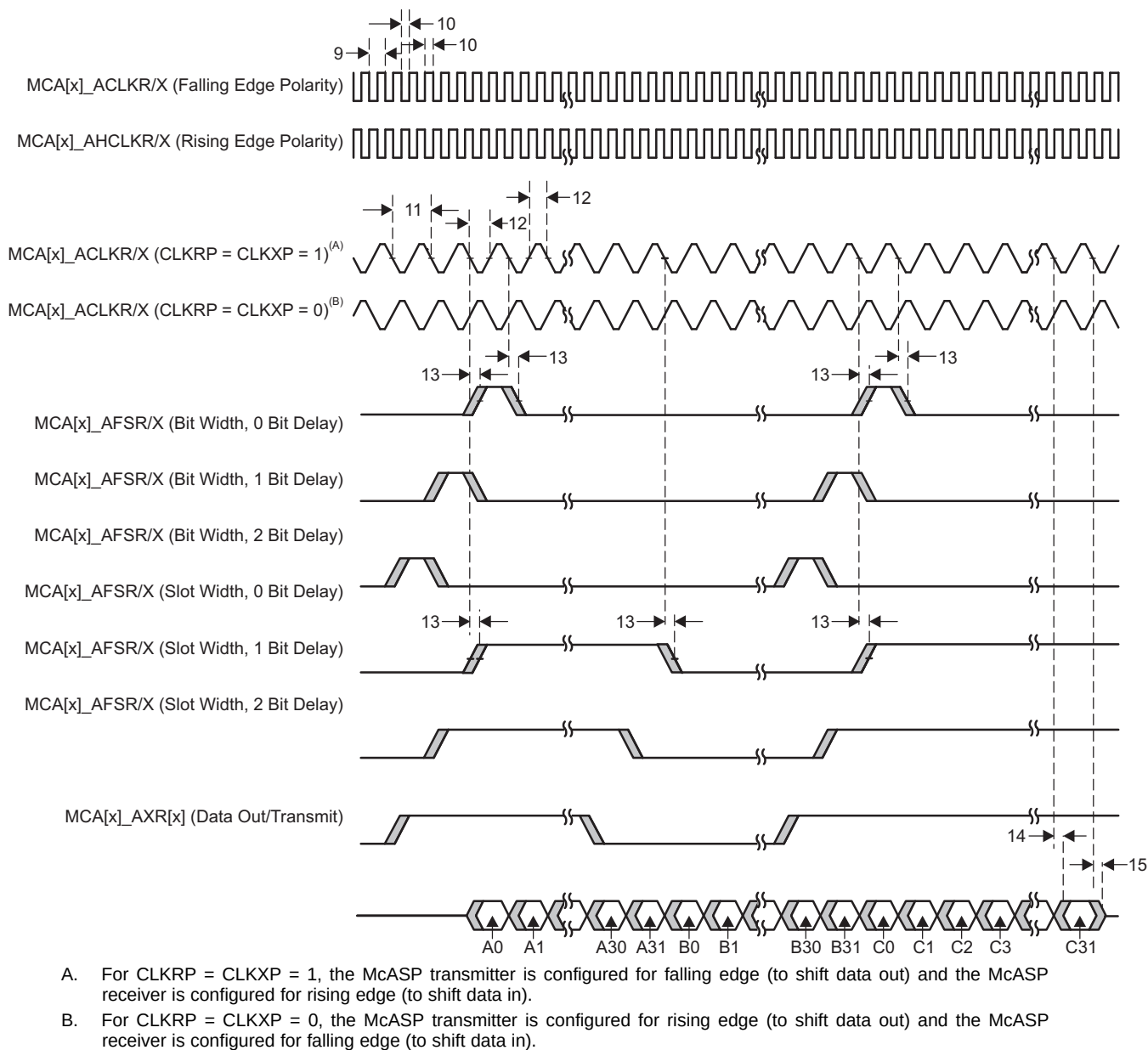
Figure 9-82. McASP Output Timing
