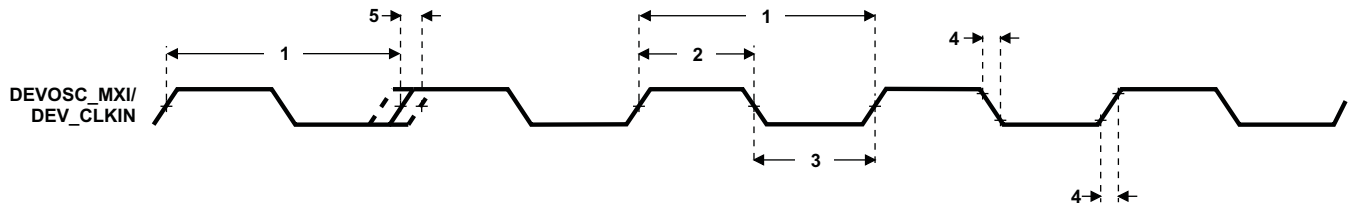
Figure 8-12. DEV_MXI/DEV_CLKIN Timing
