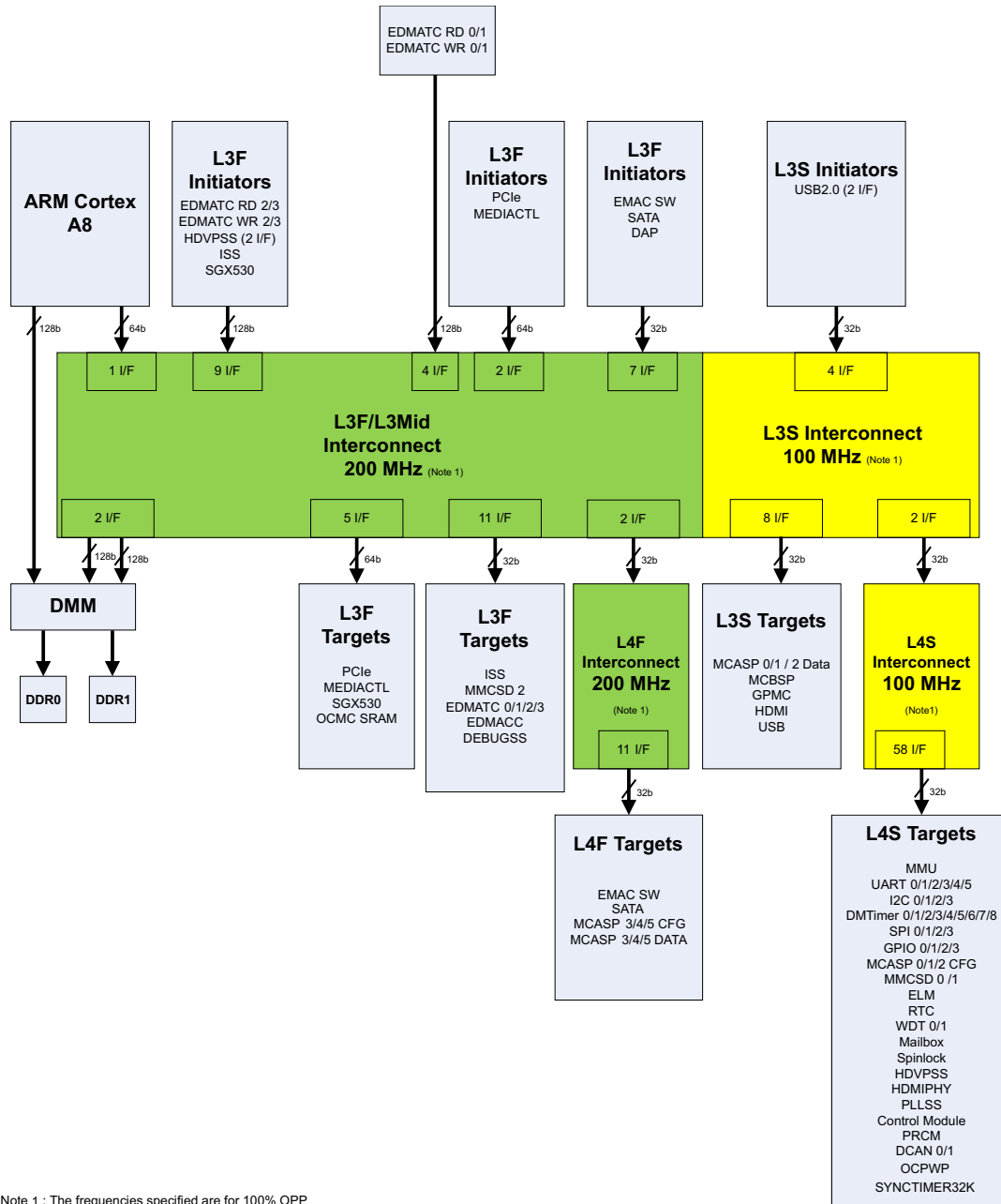
Figure 6-1. System Interconnect
