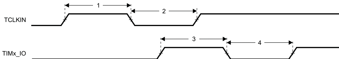
Figure 9-94. Timer Timing
