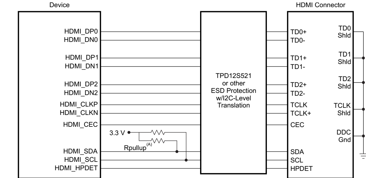
Figure 9-37. HDMI Interface High-Level Schematic
