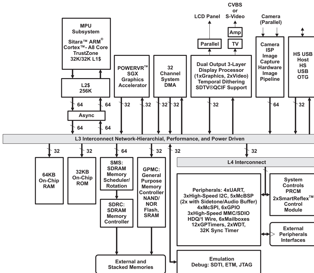
Figure 1-1. AM3715/03 Functional Block Diagram
