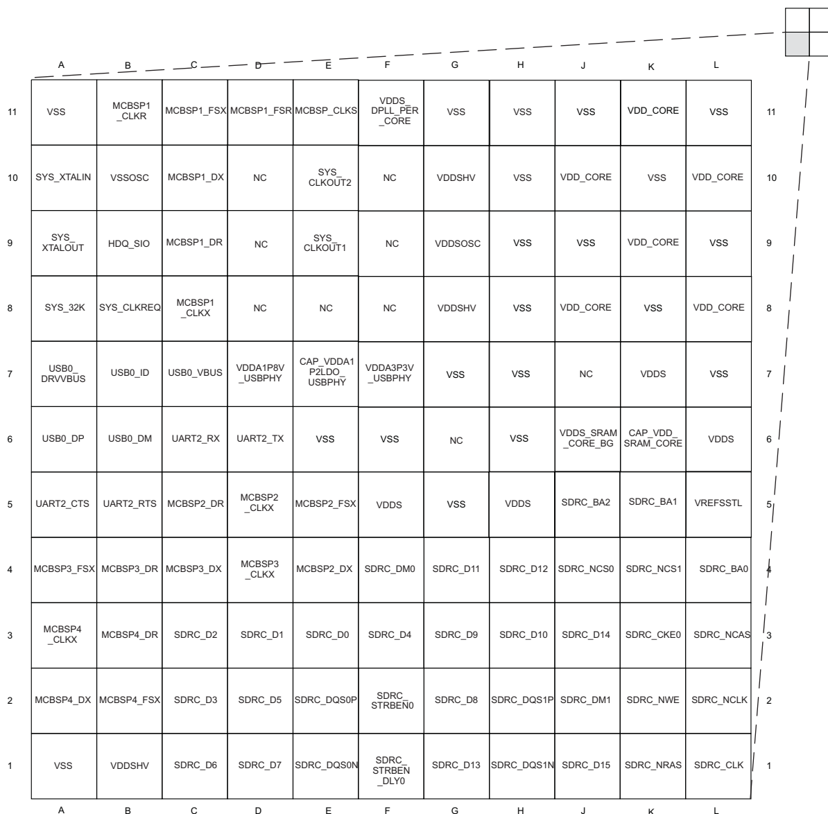
Figure 4-7. ZER Pin Map [Quadrant C]
