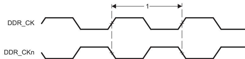
図 7-38. DDR2 Memory Interface Clock Timing
