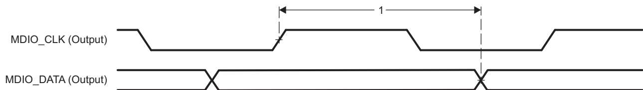
図 7-104. PRU-ICSS MDIO_DATA Timing – Output Mode
