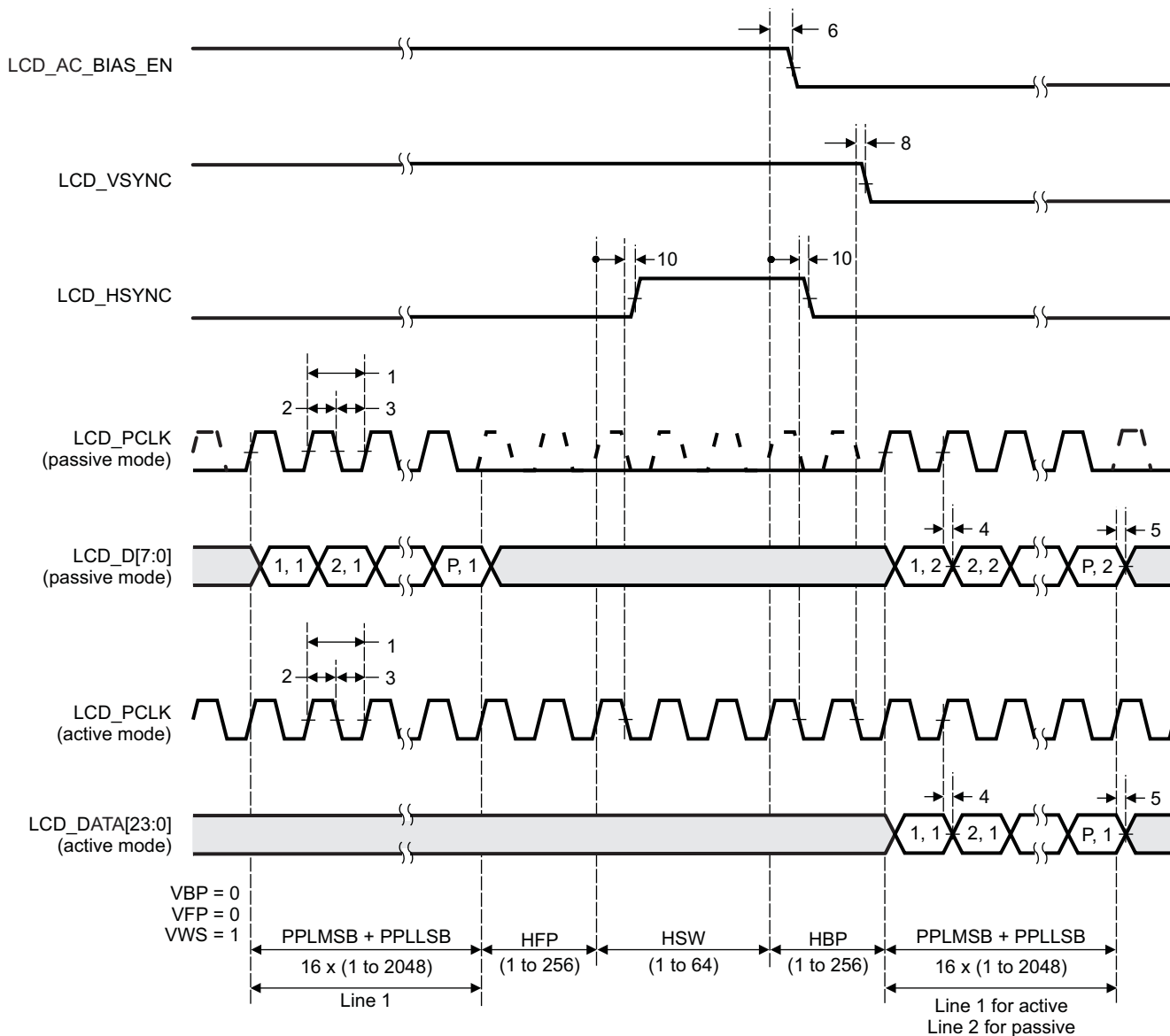
7-85. LCD Raster-Mode Control Signal Deactivation
