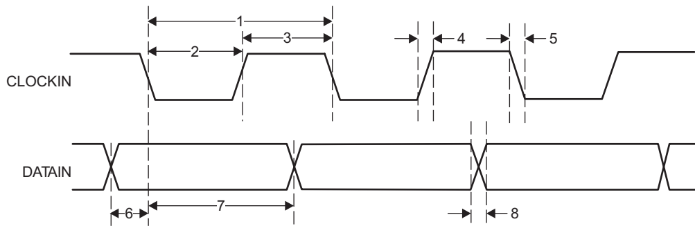
図 7-99. PRU-ICSS PRU Parallel Capture Timing - Falling Edge Mode
