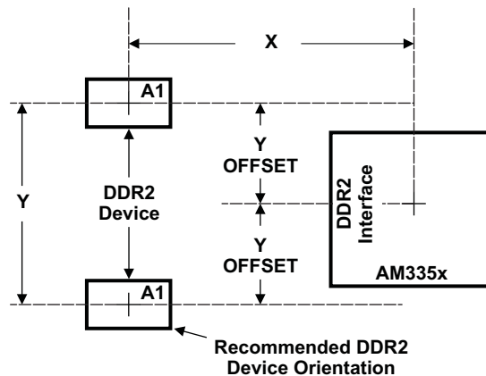
7-41. AM335x Device and DDR2 Device Placement
