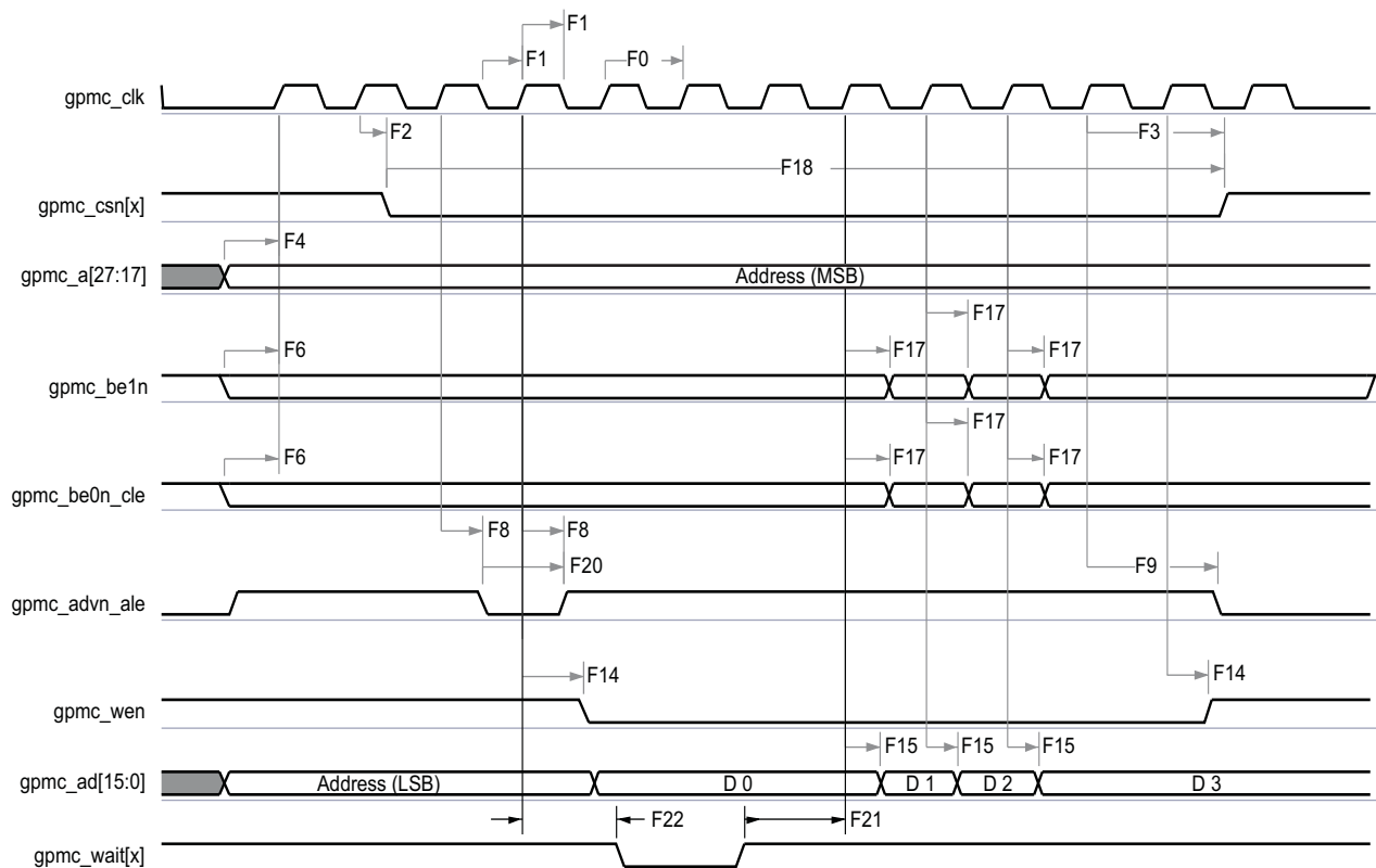
7-21. GPMC and Multiplexed NOR Flash—Synchronous Burst Write
