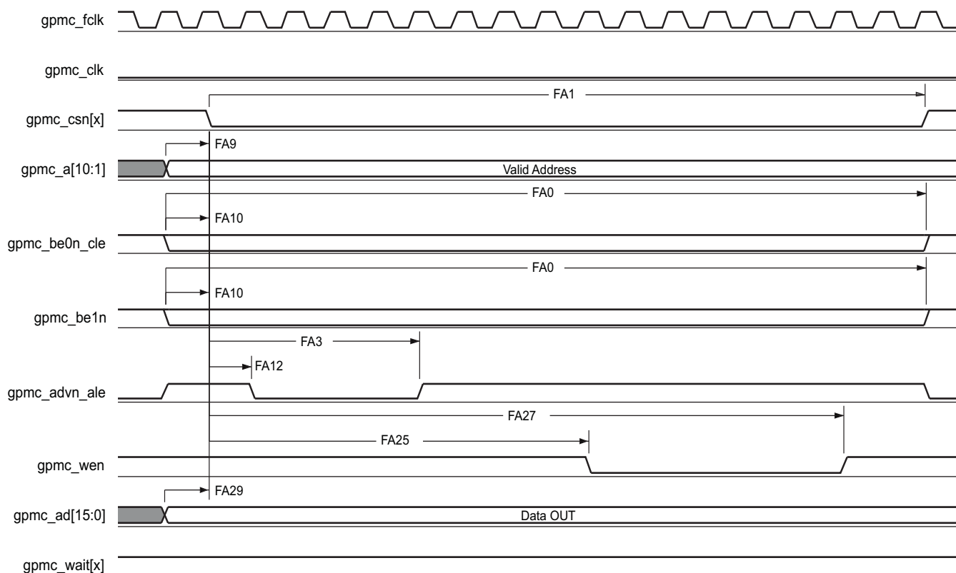
FIG 7-25. GPMC and NOR Flash—Asynchronous Write—Single Word
