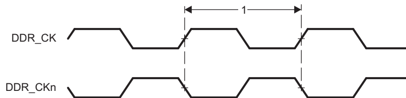
図 7-32. LPDDR Memory Interface Clock Timing
