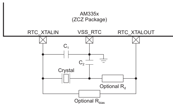
FIG 6-12. OSC1 (ZCE Package) Crystal Circuit Schematic
