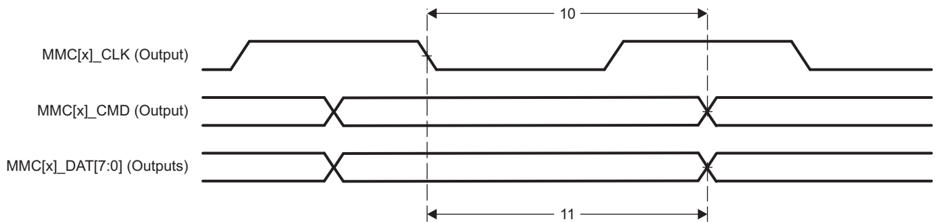
図 7-94. MMC[x]_CMD and MMC[x]_DAT[7:0] Output Timing—Standard Mode
