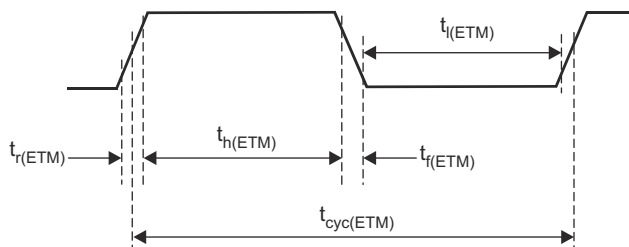
図 6-24. ETMTRACECLKOUT Timing
