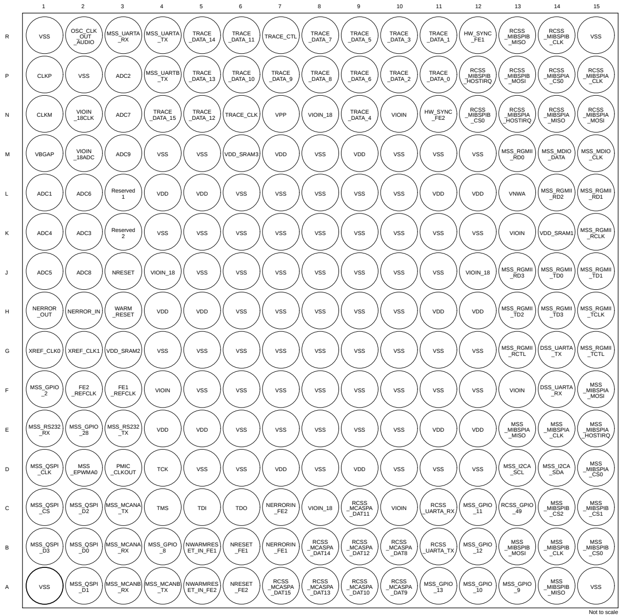
☒ 5-2. NZN NZN0225A Pin Diagram (Bottom View)
