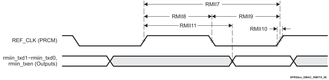
図 6-13. GMAC Transmit Interface Timing RMIIn Operation
