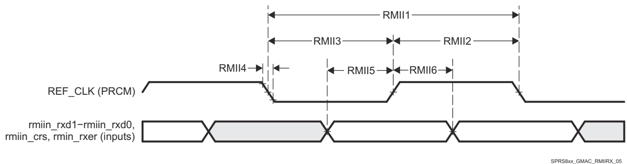
図 6-14. GMAC Receive Interface Timing RMIIn operation
