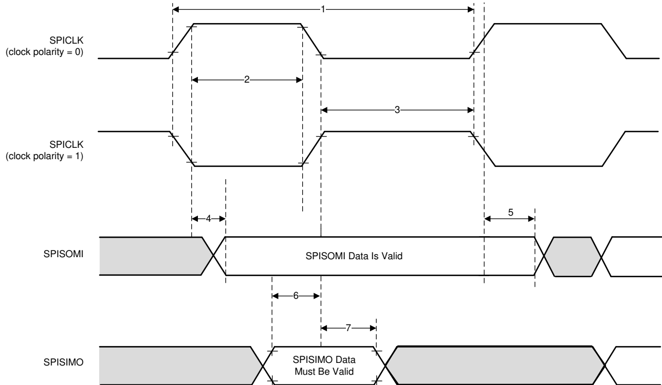
図 6-9. SPI Slave Mode External Timing (CLOCK PHASE = 0)
