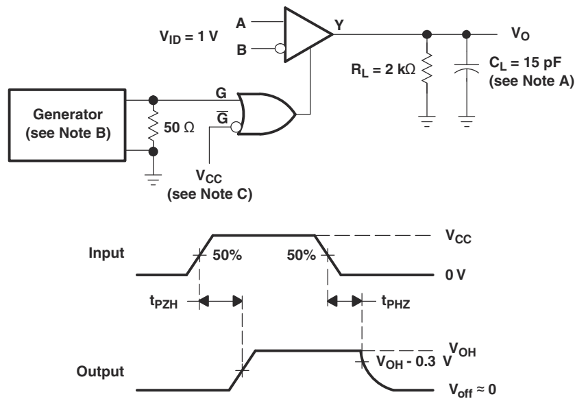
7-1. Switching Test Circuit and Voltage Waveforms
