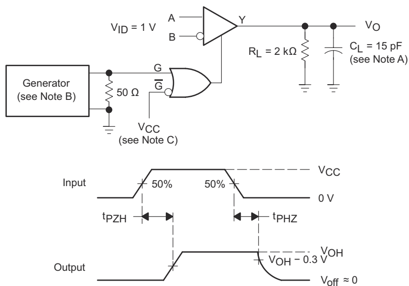
FIG 7-1. t_{PLH} and t_{PHL} Test Circuit and Voltage Waveforms
