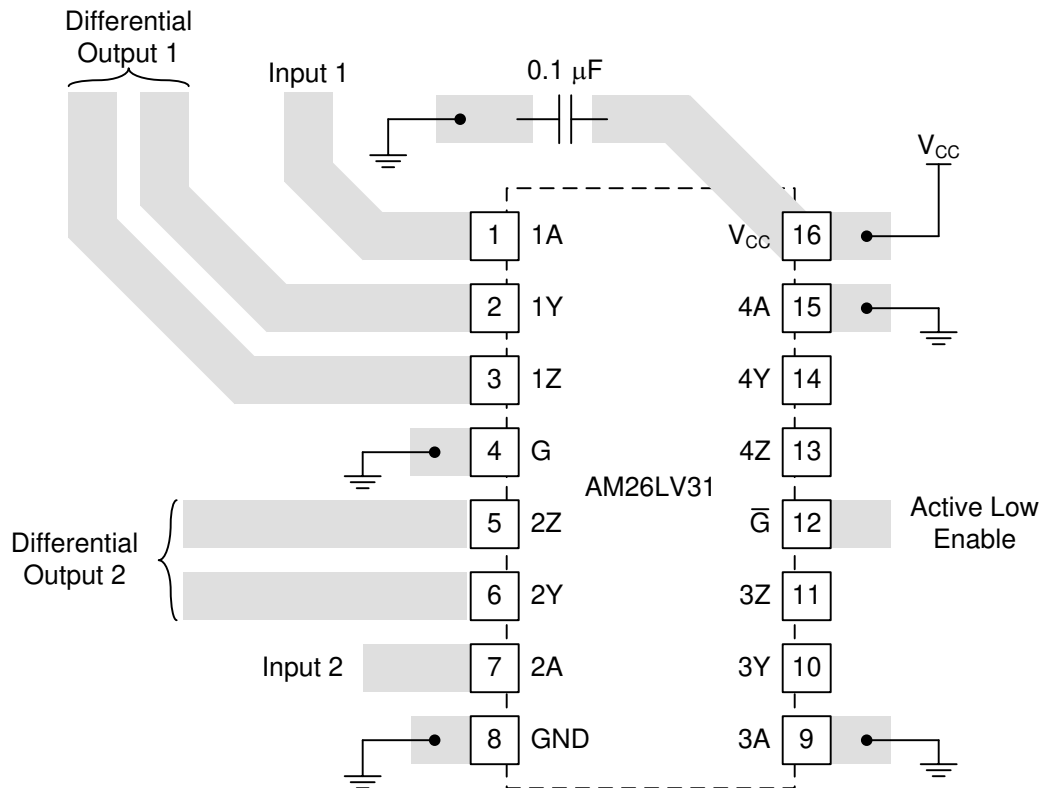
図 8-3. Trace Layout on PCB and Recommendations
