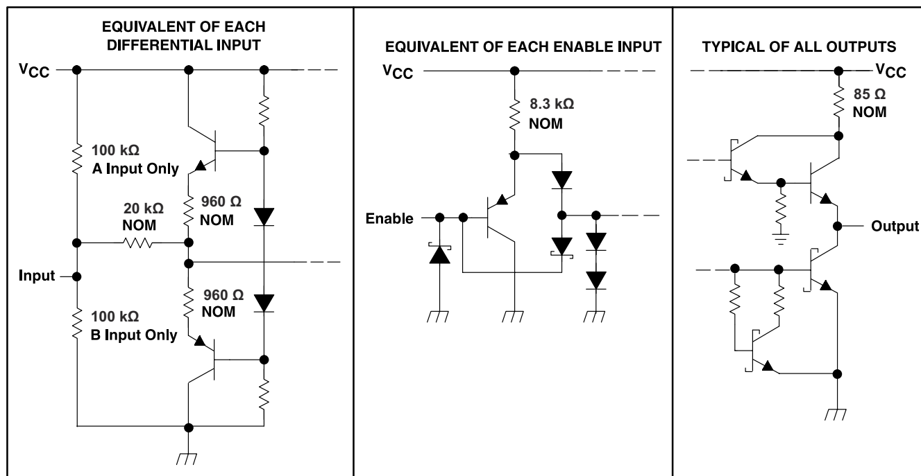
7-5. Schematics of Inputs and Outputs
