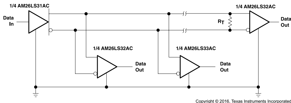
9-1. Application Diagram
