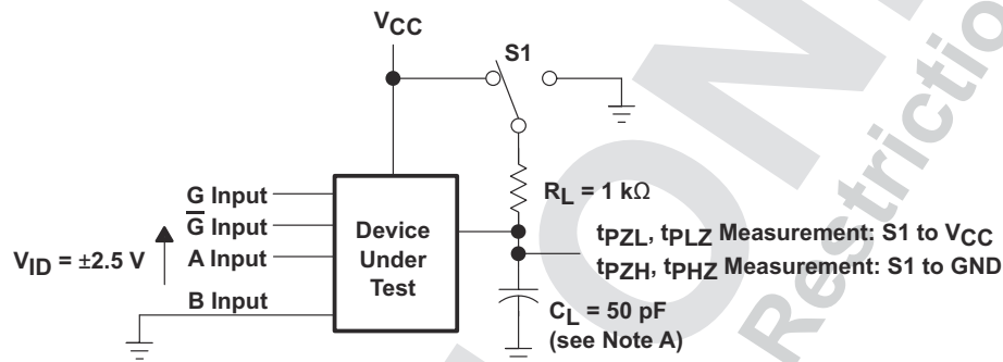
TEST CIRCUIT
