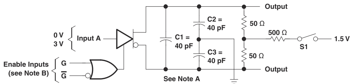
TEST CIRCUIT
