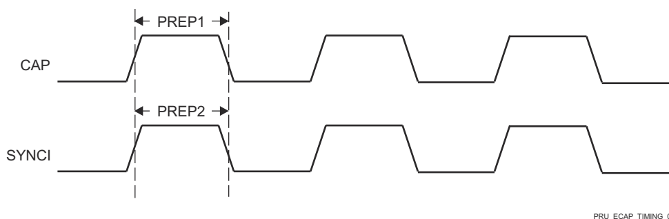
FIG 6-57. PRU-ICSS ECAP Timing
