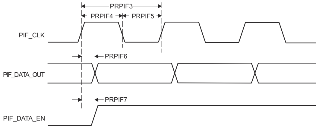
6-51. PRU-ICSS PRU Peripheral Interface Switching Characteristics
