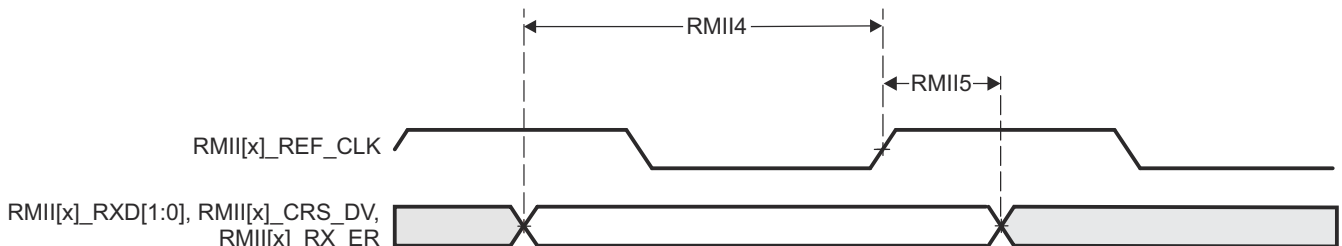
FIG 6-12. CPSW RMII[x]_RXD[1:0], RMII[x]_CRS_DV, RMII[x]_RX_ER Timing Requirements – RMII Mode
