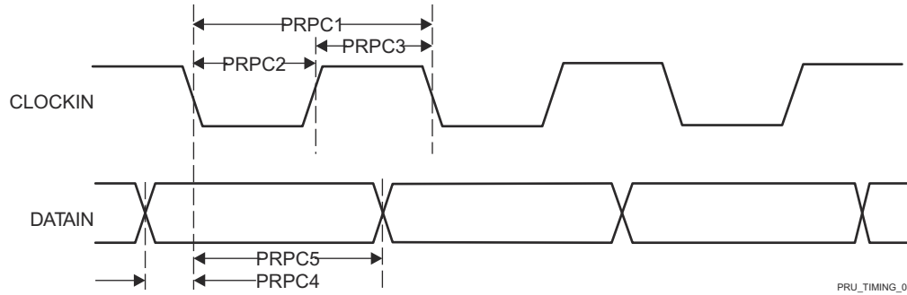
図 6-45. PRU-ICSS PRU Parallel Capture Timing Requirements – Falling Edge Mode
