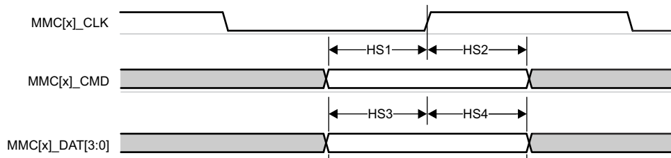
図 6-30. MMC – High Speed – Receive Mode
