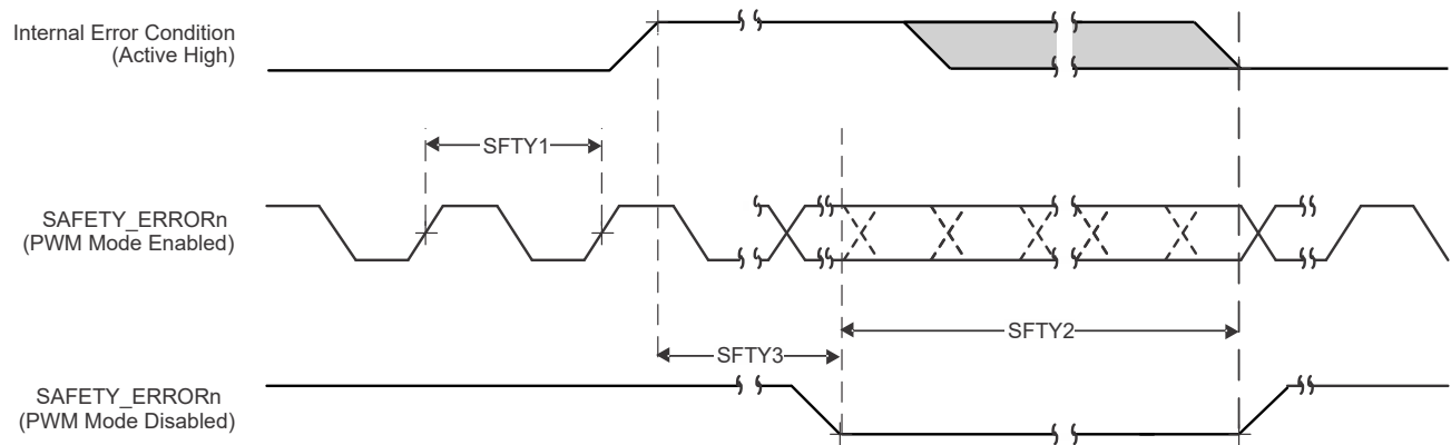
図 6-7. MCU_SAFETY_ERRORn Timing Requirements and Switching Characteristics
