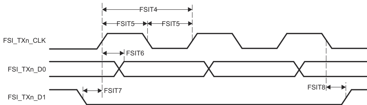
図 6-23. FSI Switching Characteristics - SPI Mode
