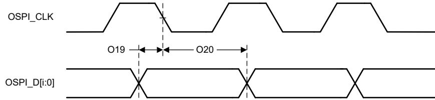
図 6-34. OSPI0 Timing Requirements – PHY SDR with Internal PHY Loopback
