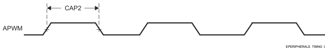
6-15. ECAP Switching Characteristics
