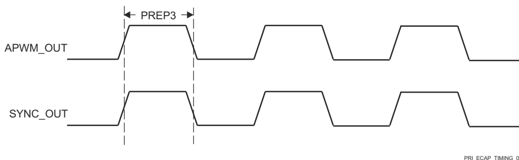
FIG 6-58. PRU-ICSS ECAP Switching Characteristics
