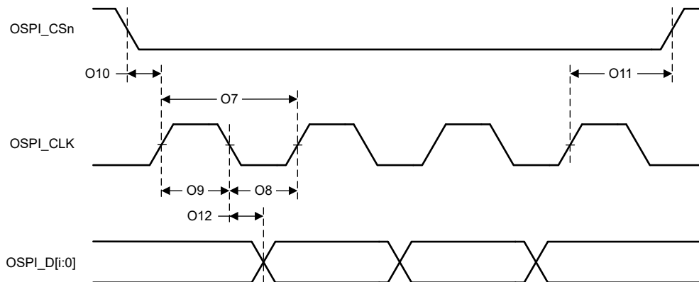
図 6-36. OSPI0 Switching Characteristics – PHY SDR
