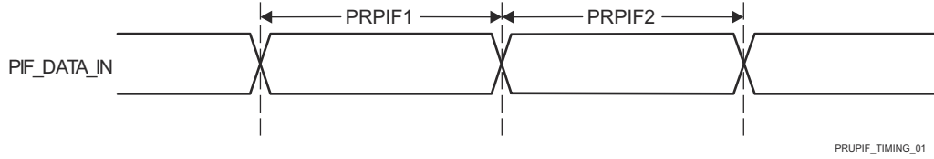
6-50. PRU-ICSS PRU Peripheral Interface Timing Requirements
