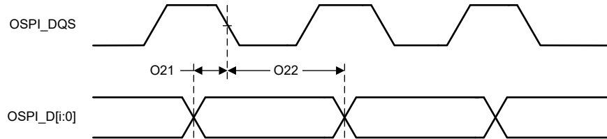
図 6-35. OSPI0 Timing Requirements – PHY SDR with External Board Loopback
