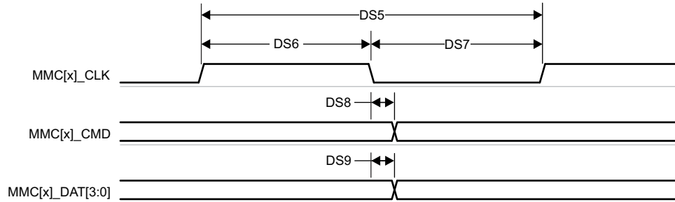
図 6-29. MMC – Default Speed – Transmit Mode
