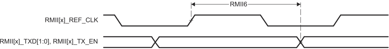
図 6-13. CPSW RMII[x]_TXD[1:0], and RMII[x]_TX_EN Switching Characteristics – RMII Mode
