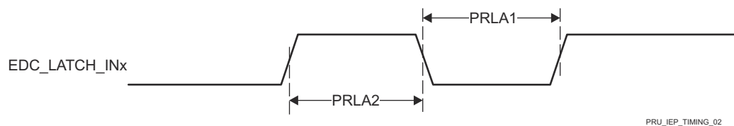
6-55. PRU-ICSS IEP LATCH_INx Timing Requirements
