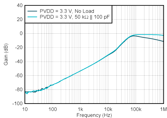
図 5-27. DAC AC PSRR vs Frequency
