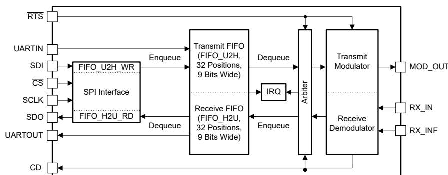
Figure 6-17. HART Architecture
