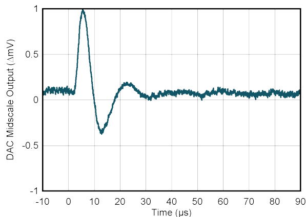
PVDD = 5.5 V
