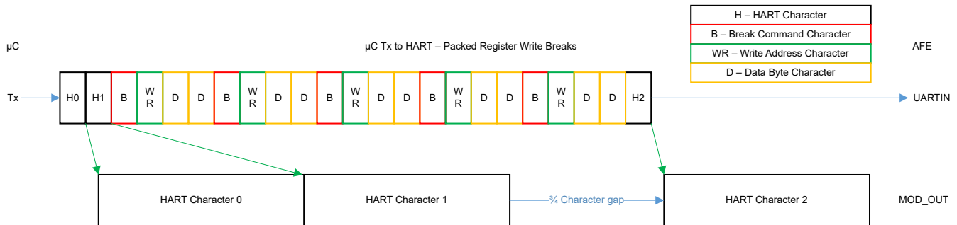
図 6-35. Packed HART Transmit With UBM Register Writes
