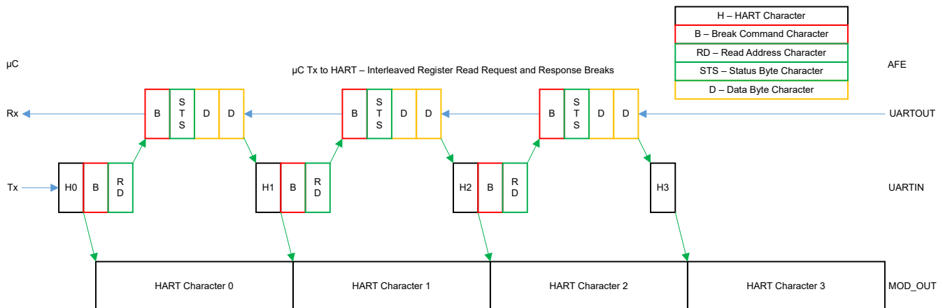
図 6-36. Interleaved HART Transmit With UBM Register Read Requests and Responses
