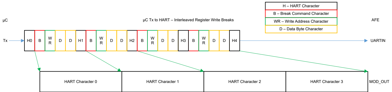
図 6-34. Interleaved HART Transmit With UBM Register Writes
