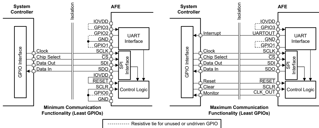
図 6-17. SPI Mode Connections
