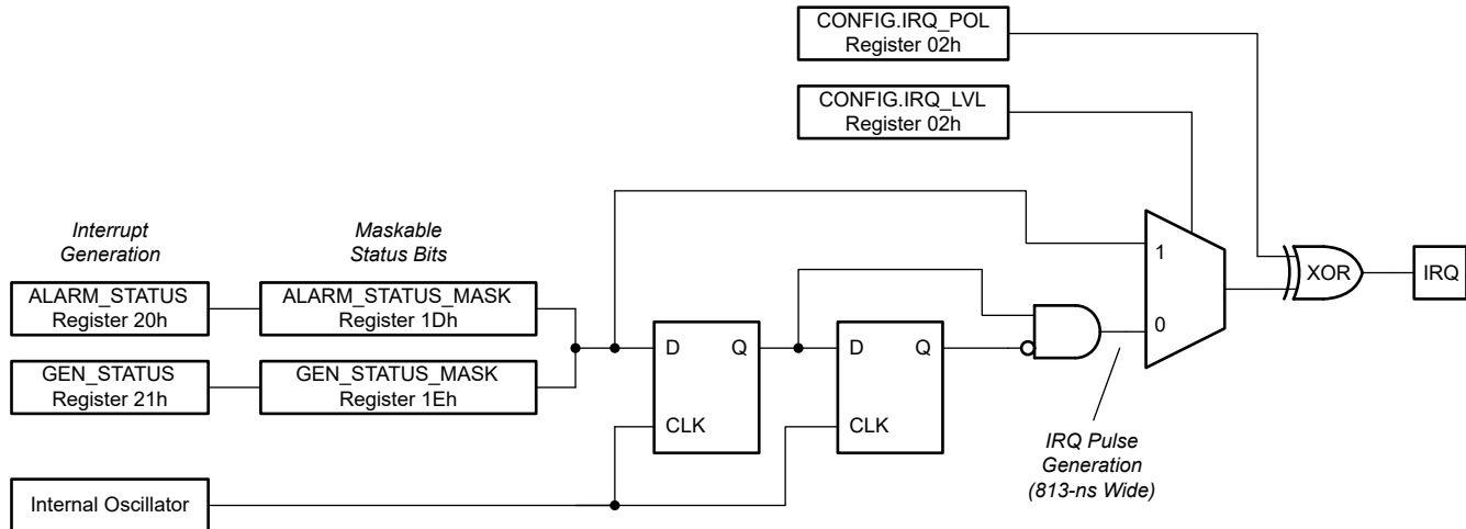
6-15. IRQ Block Diagram
