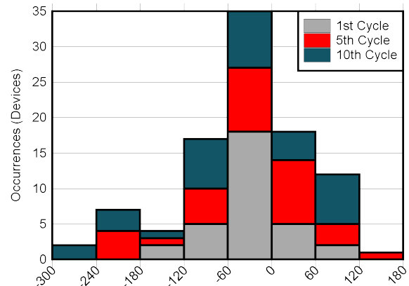
25°C Reference Voltage Temperature Cycle Hysteresis (ppm)
