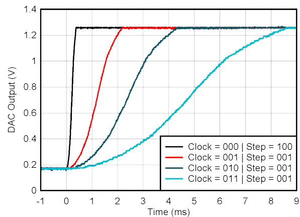
6-24. DAC Settling Time With Sinusoidal Slew Rate Control
