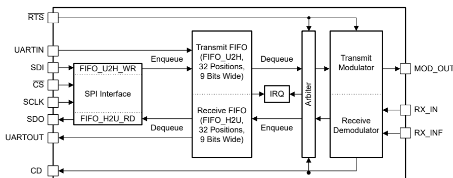
Figure 7-17. HART Architecture
