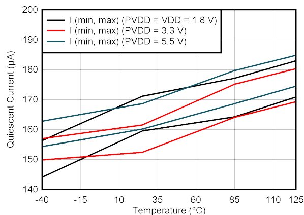
FIG 6-51. PVDD Supply Current vs Temperature
