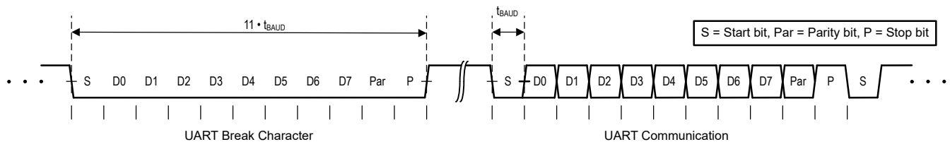
6-2. UBM Timing
