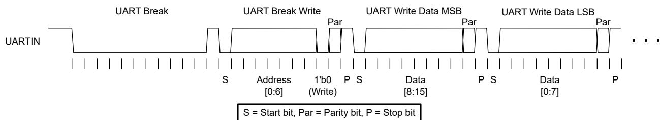
Figure 7-21. UARTIN Break Write Data Format
