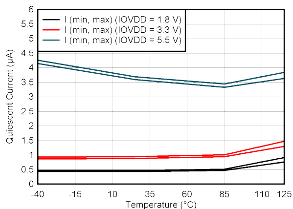
FIG 6-52. IOVDD Supply Current vs Temperature
