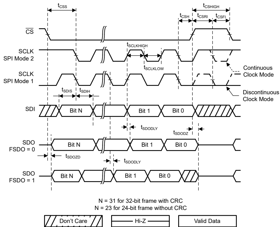
6-1. SPI Timing
