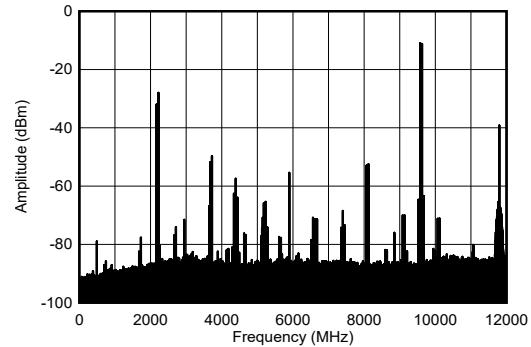
図 4-270. TX Single Tone Spectrum at 9.61GHz and -12dBFS (wideband)
