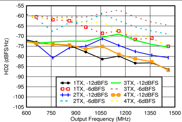
Matching at 0.8GHz, f_{\text{DAC}} = 5898.2\text{GSPS} , straight mode
