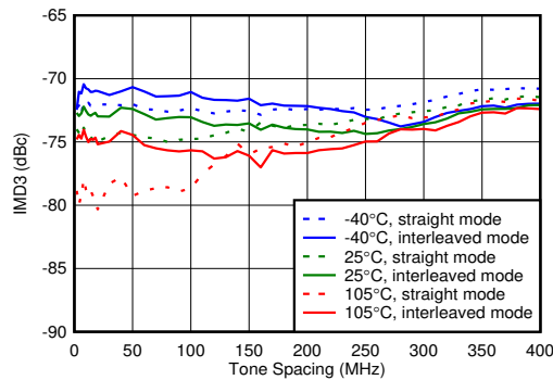
FIG 4-99. TX IMD3 vs Tone Spacing and Temperature at 2.6GHz
