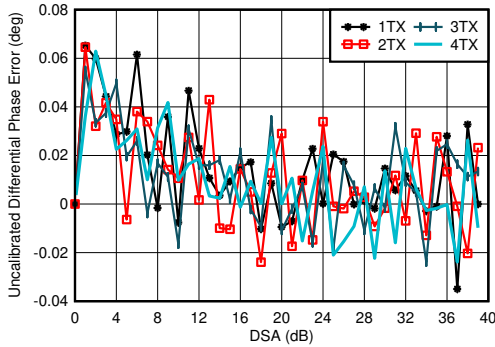
FIG 4-124. TX Uncalibrated Differential Phase Error vs DSA Setting and Channel at 3.5GHz
