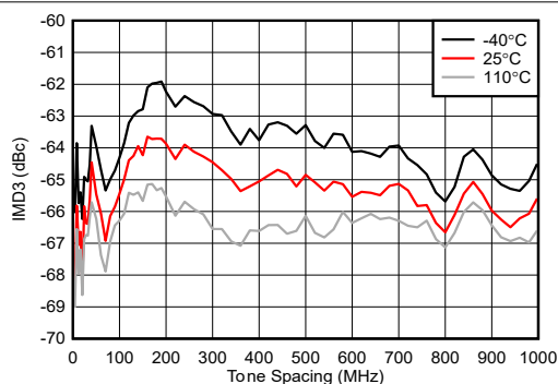
FIG 4-259. TX IMD3 vs Tone Spacing at 9.61GHz
