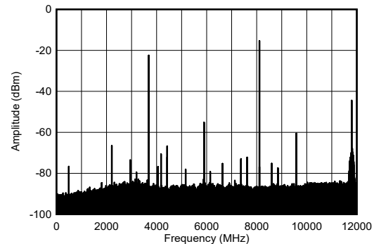
FIG 4-205. TX Single Tone Output Spectrum at 8.1GHz
