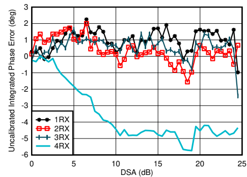
FIG 4-400. RX Uncalibrated Differential Phase Error vs DSA Setting at 4.9GHz
