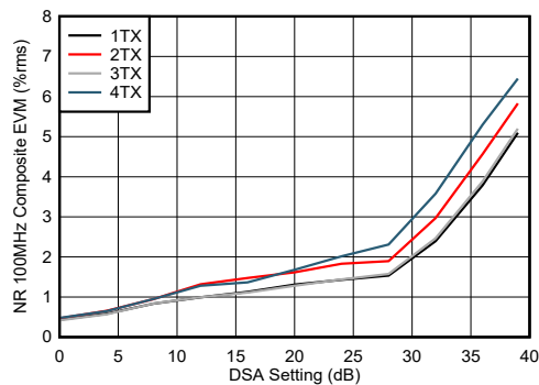
FIG 4-228. TX NR100MHz EVM vs DSA Setting 8.1GHz
