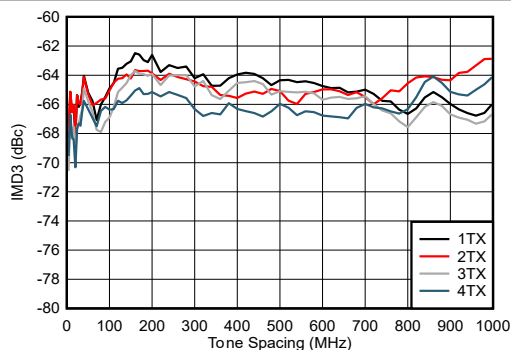
FIG 4-257. TX IMD3 vs Tone Spacing at 9.61GHz
