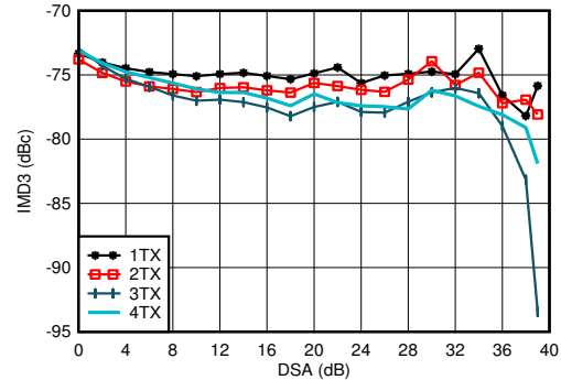
FIG 4-97. TX IMD3 vs DSA Setting at 2.6GHz
