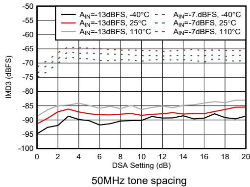
4-430. RX IMD3 vs DSA Setting at 8.1GHz
