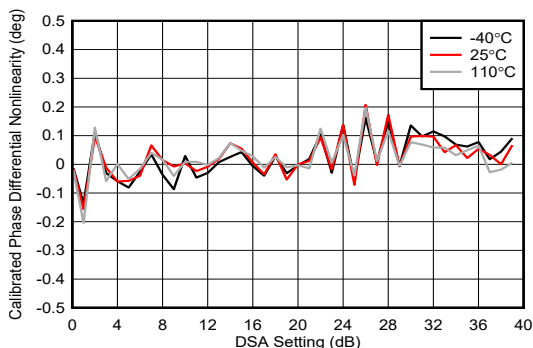
FIG 4-198. TX DSA Calibrated Phase Differential Nonlinearity at 8.1GHz
