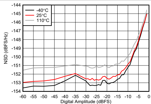
FIG 4-261. TX NSD vs Digital Amplitude at 9.61GHz
