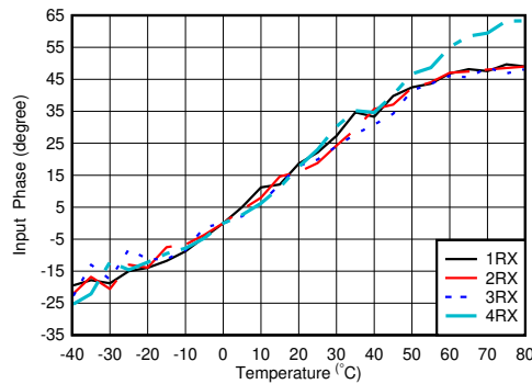
FIG 4-395. RX Input Phase vs Temperature and DSA at f_{\text{OUT}} = 4.9\text{GHz}
