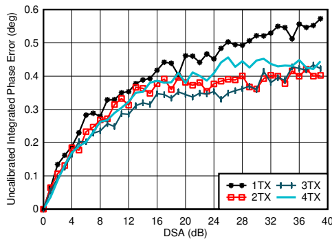
FIG 4-126. TX Uncalibrated Integrated Phase Error vs DSA Setting and Channel at 3.5GHz
