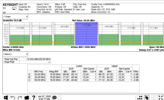
4-174. TX 20MHz LTE Output Spectrum at 4.9GHz
