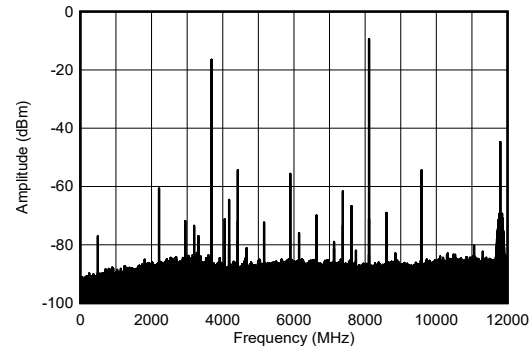
FIG 4-203. TX Single Tone Output Spectrum at 8.1GHz
