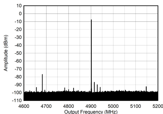
✎ 5-516. TX Single Tone (-1 dBFS) Output Spectrum at 4.9 GHz ( \pm 300\text{ MHz} )
