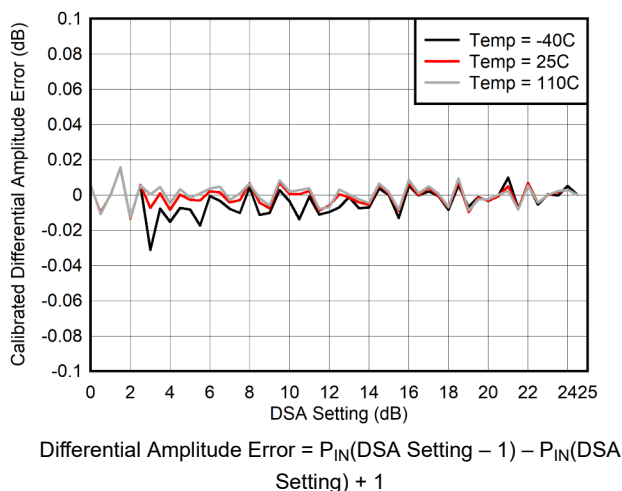
图 5-31. RX Calibrated Differential Amplitude Error vs DSA Setting at 400 MHz
