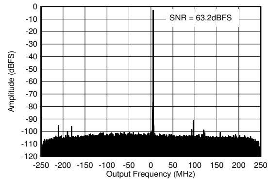
Figure 5-61. RX Output FFT at 0.8 GHz
