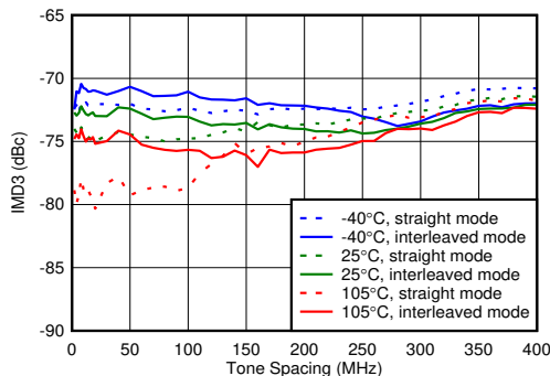
FIG 5-377. TX IMD3 vs Tone Spacing and Temperature at 2.6 GHz
