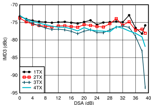
FIG 5-375. TX IMD3 vs DSA Setting at 2.6 GHz
