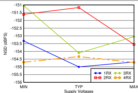
FIG 5-110. RX Noise Spectral Density vs Supply and Channel at 1.75 GHz
