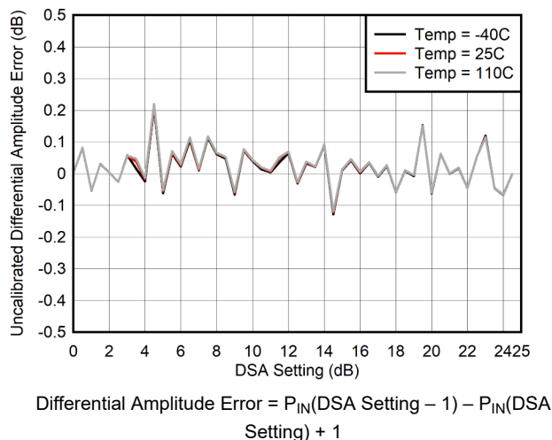
图 5-30. RX Uncalibrated Differential Amplitude Error vs DSA Setting at 30 MHz
