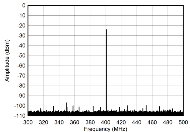
5-255. Single Tone Spectrum at 400 MHz and -30 dBFS (±100MHz)
