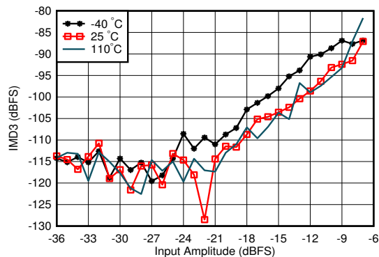
5-189. RX IMD3 vs Input Level and Temperature at 4.9 GHz
