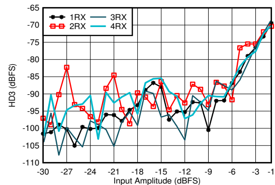
5-196. RX HD3 vs Input Level and Channel at 4.9 GHz
