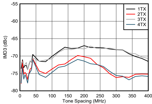
5-446. TX IMD3 vs Tone Spacing and Channel at 3.75GHz
