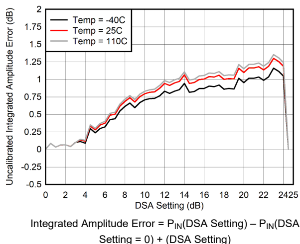
图 5-32. RX Uncalibrated Integrated Amplitude Error vs DSA Setting at 400 MHz
