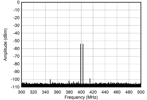
5-265. Dual Tone Spectrum at 400 MHz and -60 dBFS (±100MHz)
