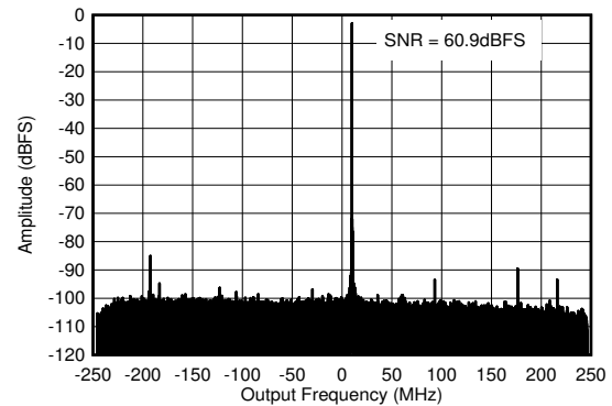
Figure 5-92. RX Output FFT at 1.75 GHz
