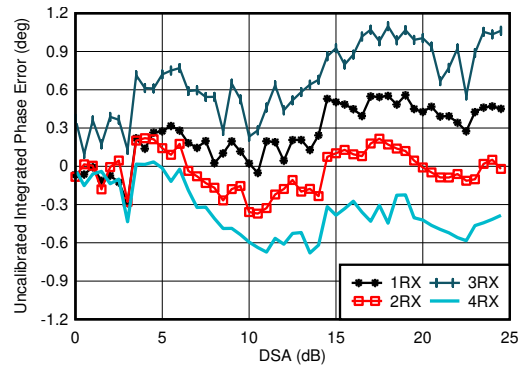
FIG 5-57. RX Uncalibrated Differential Phase Error vs DSA Setting at 0.8 GHz
