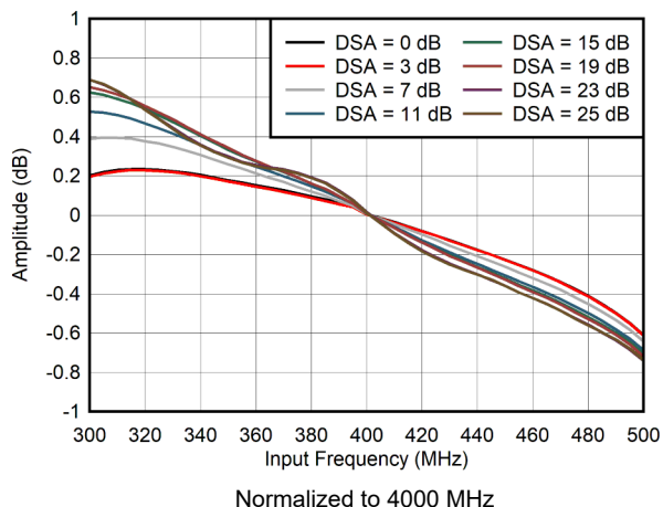
图 5-29. RX In-Band Gain Flatness, f_{\text{IN}} = 400\text{ MHz}
