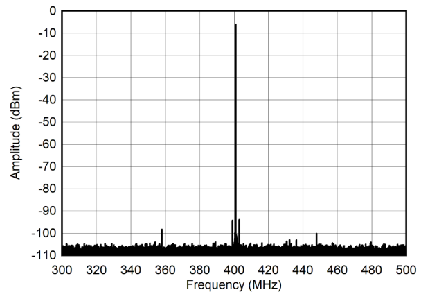
5-253. Single Tone Spectrum at 400 MHz and -12 dBFS (±100MHz)
