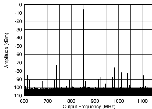
f_{\text{DAC}} = 5898.24\text{MSPS} , interleave mode, 0.8 GHz matching, includes PCB and cable losses
