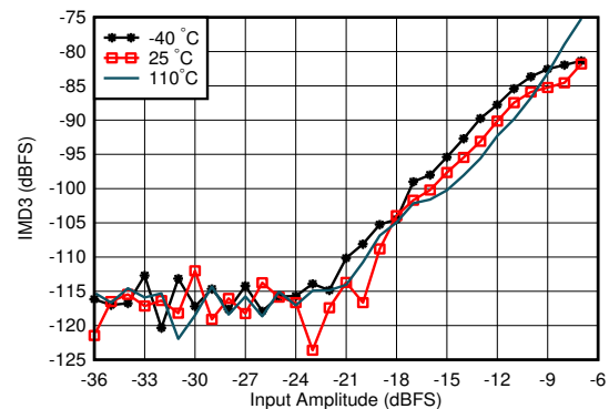
5-190. RX IMD3 vs Input Level and Temperature at 4.9 GHz
