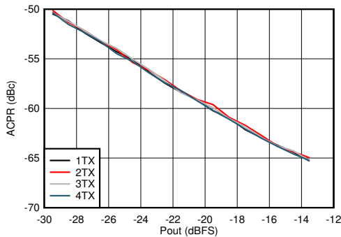
5-383. TX 20-MHz LTE alt-ACPR vs Digital Level at 2.6 GHz
