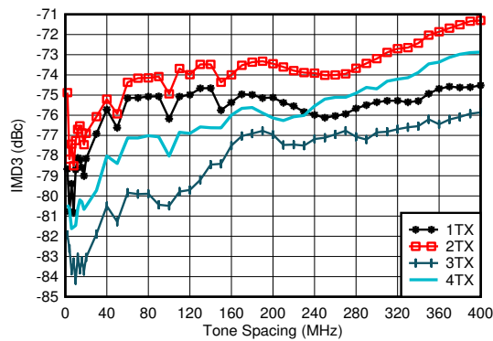
5-298. TX IMD3 vs Tone Spacing and Channel at 0.85 GHz
