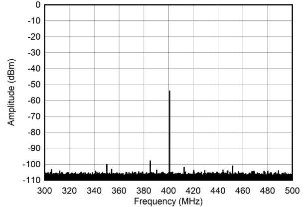
FIG 5-257. Single Tone Spectrum at 400 MHz and -60 dBFS (±100MHz)
