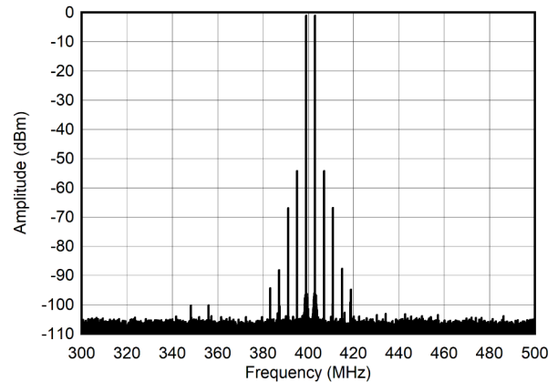
FIG 5-259. Dual Tone Spectrum at 400 MHz and -7 dBFS (±100MHz)
