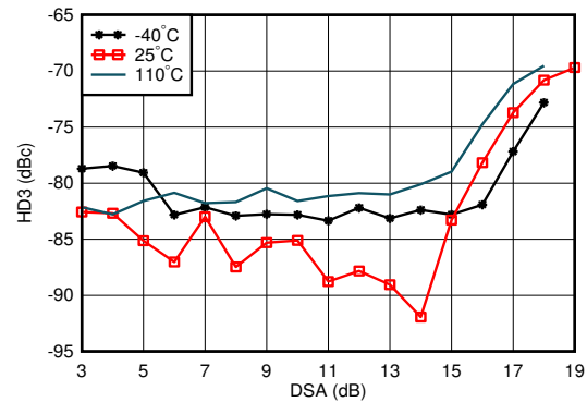
FIG 5-104. RX HD3 vs DSA Setting and Temperature at 1.9 GHz
