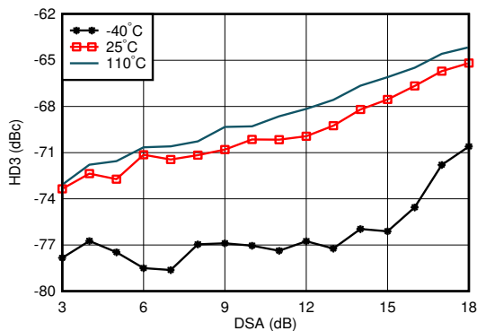
5-195. RX HD3 vs DSA Setting and Temperature at 4.9 GHz
