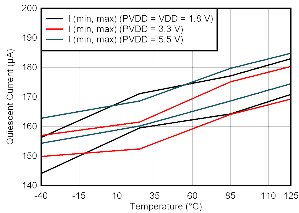
FIG 6-51. PVDD Supply Current vs Temperature
