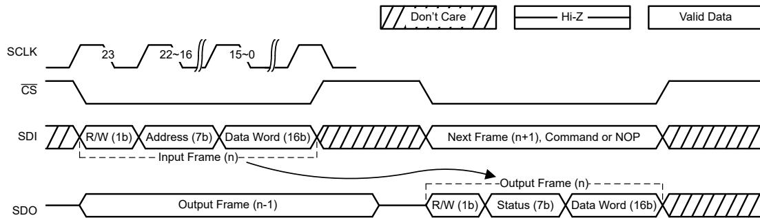
FIG 7-20. SPI Frame Details (CRC Disabled)
