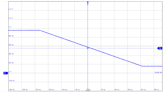
图 7-4. Linear Slew Rate: Falling
