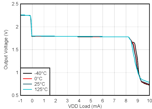
FIG 6-53. VDD Voltage vs Load Current
