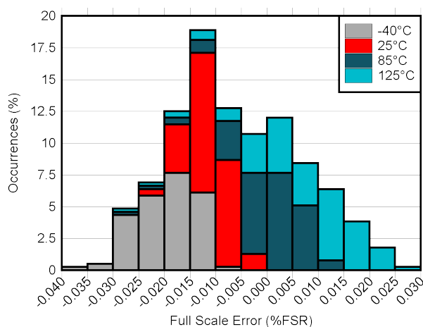
FIG 6-17. DAC Full Scale Error vs Temperature
