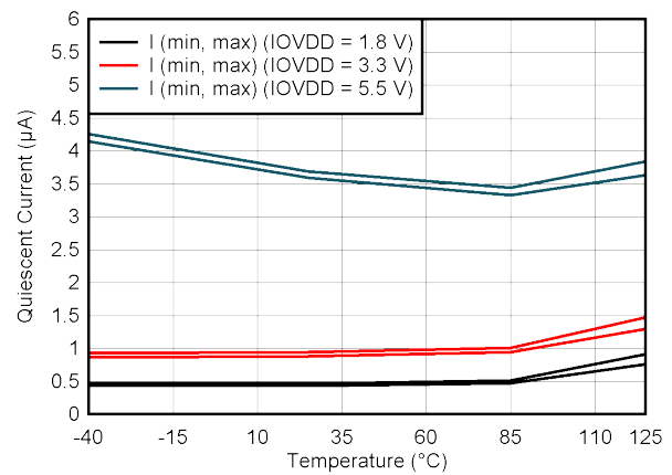
FIG 6-52. IOVDD Supply Current vs Temperature
