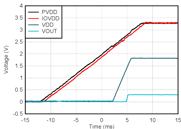
6-28. DAC Supply Power On, PVDD = 3.3\text{ V}
