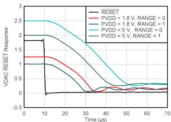
6-12. DAC RESET Response
