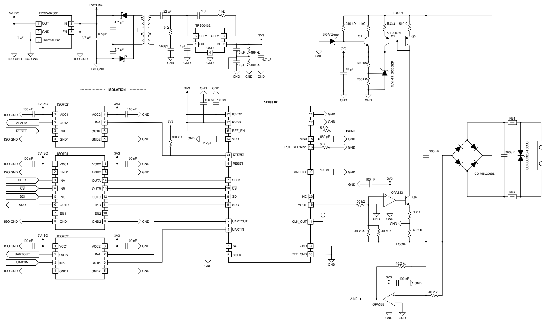
8-2. AFEx8101 in a 4-mA to 20-mA Current Transmitter
