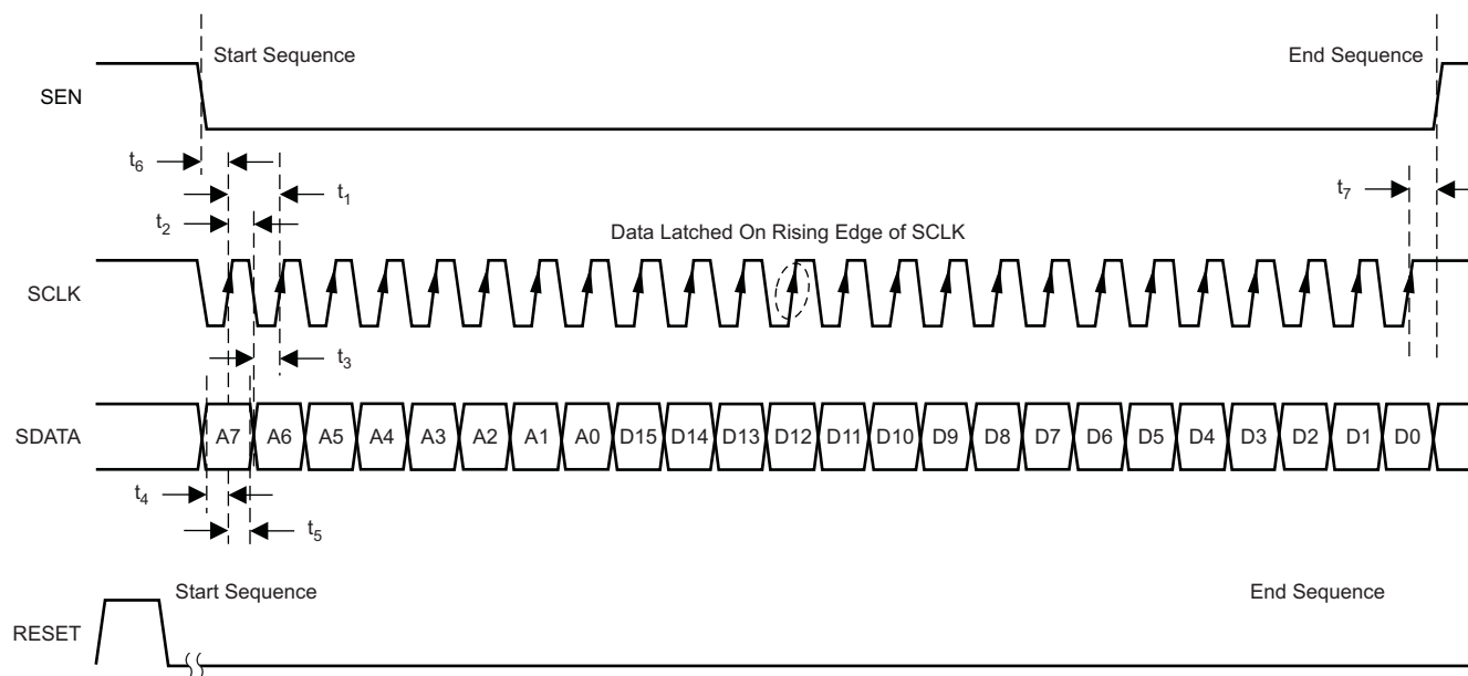
Figure 60. SPI Timing
