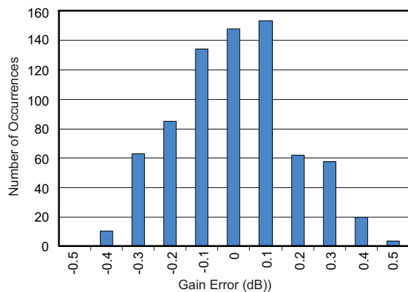
Figure 4. Gain Matching Histogram, V_{CNTL} = 0.3\text{V} (936 Channels)
