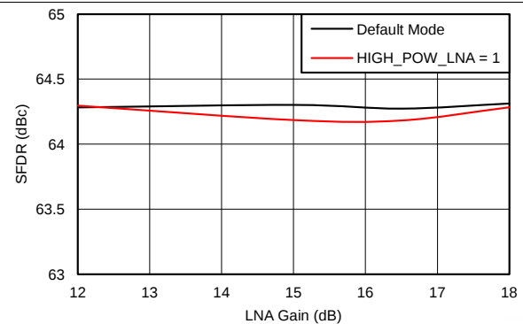
Figure 30. Spurious-Free Dynamic Range vs LNA Gain (PGA Gain = 30\text{ dB} )
