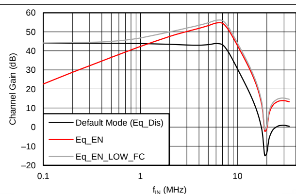
Figure 66. Filter Response (PGA Gain = 30 dB)
