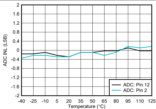
6-31. ADC INL vs Temperature
