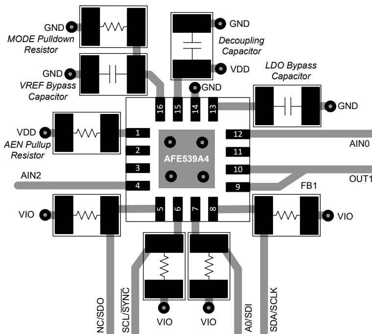
8-4. Layout Example
