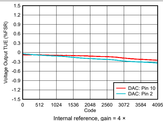
Figure 6-12. Voltage Output TUE vs Digital Input Code
