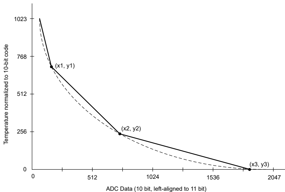
图 7-5. Thermistor Linearization
