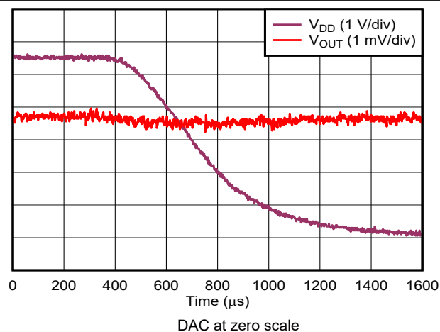
图 6-25. Voltage Output Power-Off Glitch
