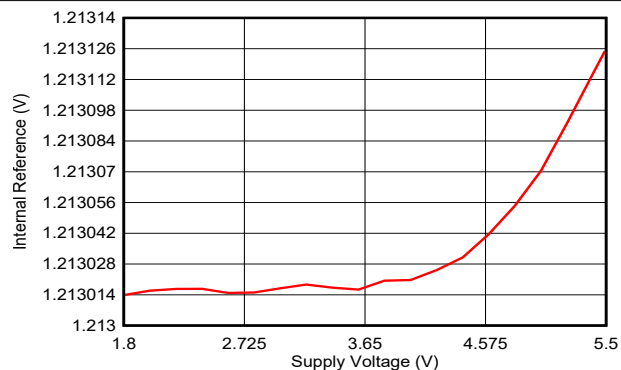
图 6-39. Internal Reference vs Supply Voltage
