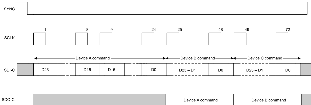
FIG 7-9. SPI Daisy-Chain Write Cycle
