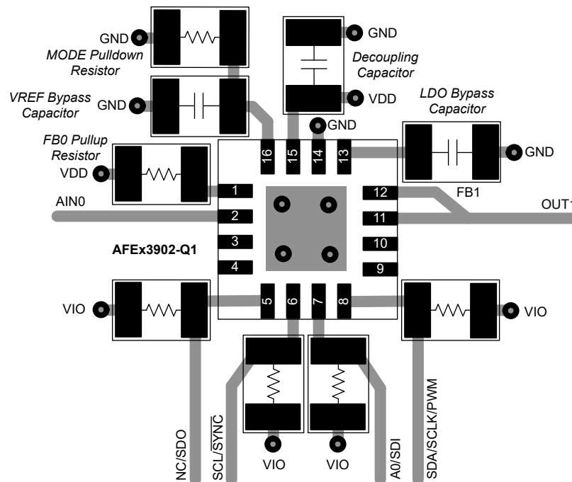
8-4. Layout Example
