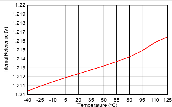
图 6-38. Internal Reference vs Temperature
