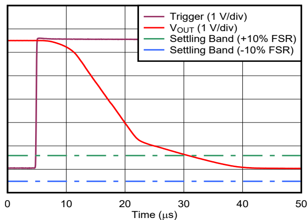
图 6-23. Voltage Output Setting Time - Falling Edge
