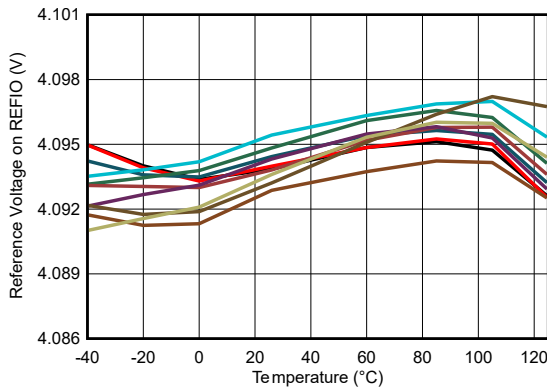
FIG 5-30. REFIO vs Temperature
