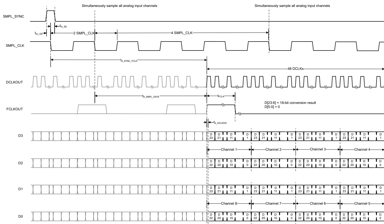
5-4. 4-SDO SDR CMOS Data Interface
