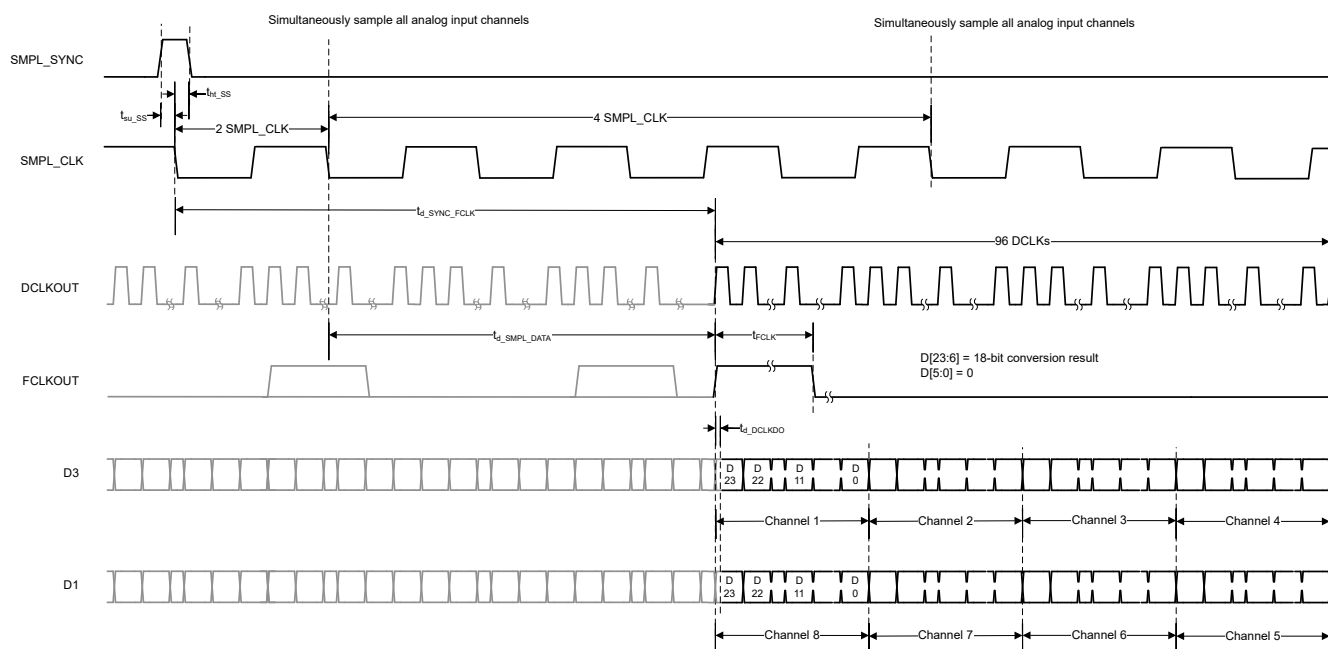
5-5. 2-SDO SDR CMOS Data Interface
