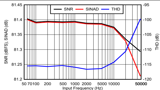
FIG 5-15. SNR, SINAD, and THD vs Input Signal Frequency
