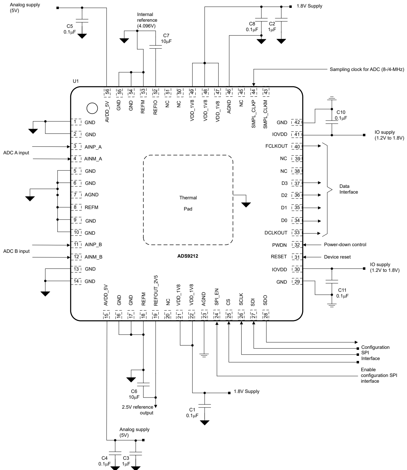
図 8-1. Typical Application
