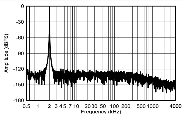
図 8-3. Typical FFT With Wide-Bandwidth LPF, RANGE = \pm 5\text{V}
