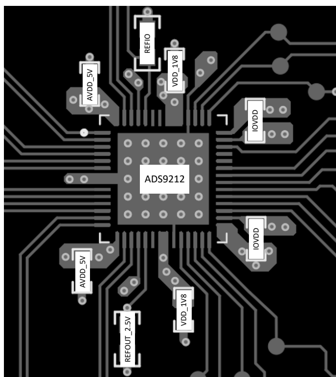
8-5. Example Layout
