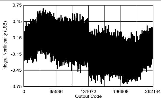
図 5-7. Typical INL With Wide-Bandwidth LPF
