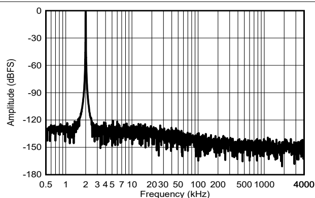
図 8-2. Typical FFT With Low-Bandwidth LPF, RANGE = \pm 5\text{V}
