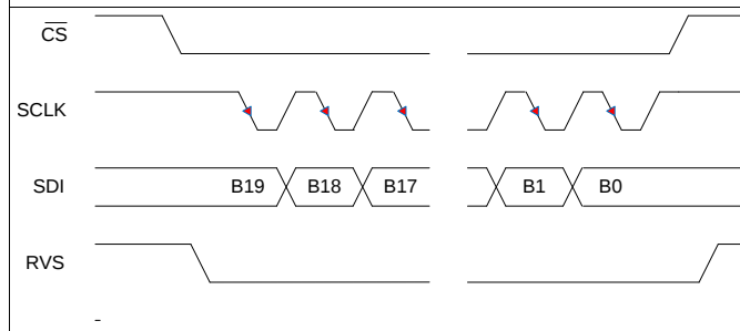
Figure 54. SPI-10-S Protocol, Optimal Command Frame
