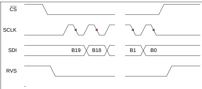
Figure 53. SPI-01-S Protocol, Optimal Command Frame
