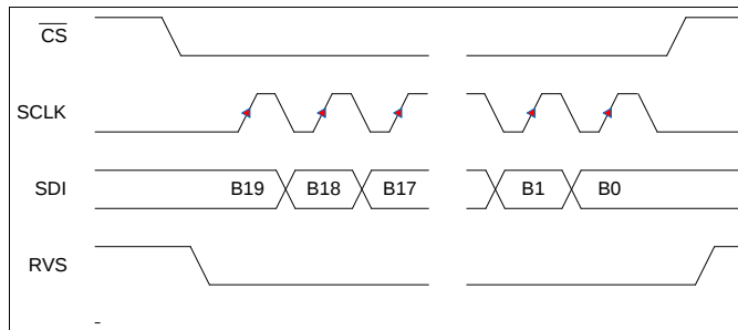
Figure 52. SPI-00-S Protocol, Optimal Command Frame
