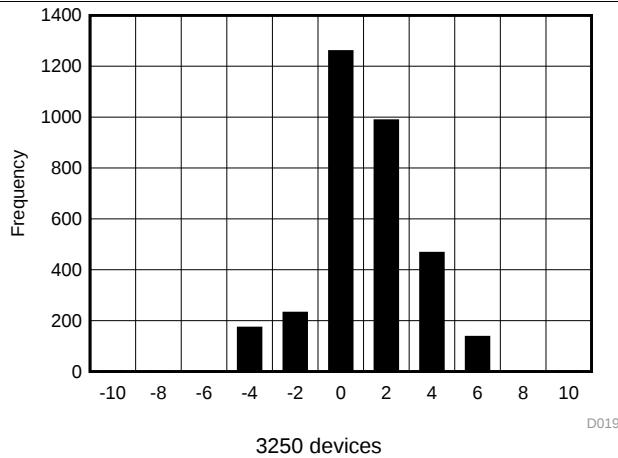
Figure 14. Typical Offset Distribution (LSB)
