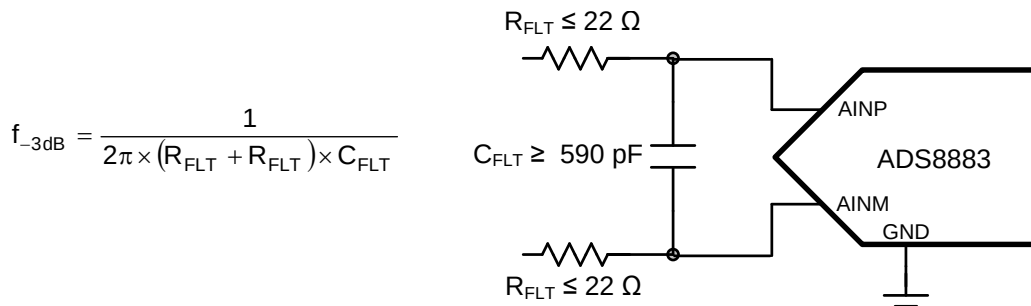
Figure 69. Antialiasing Filter
