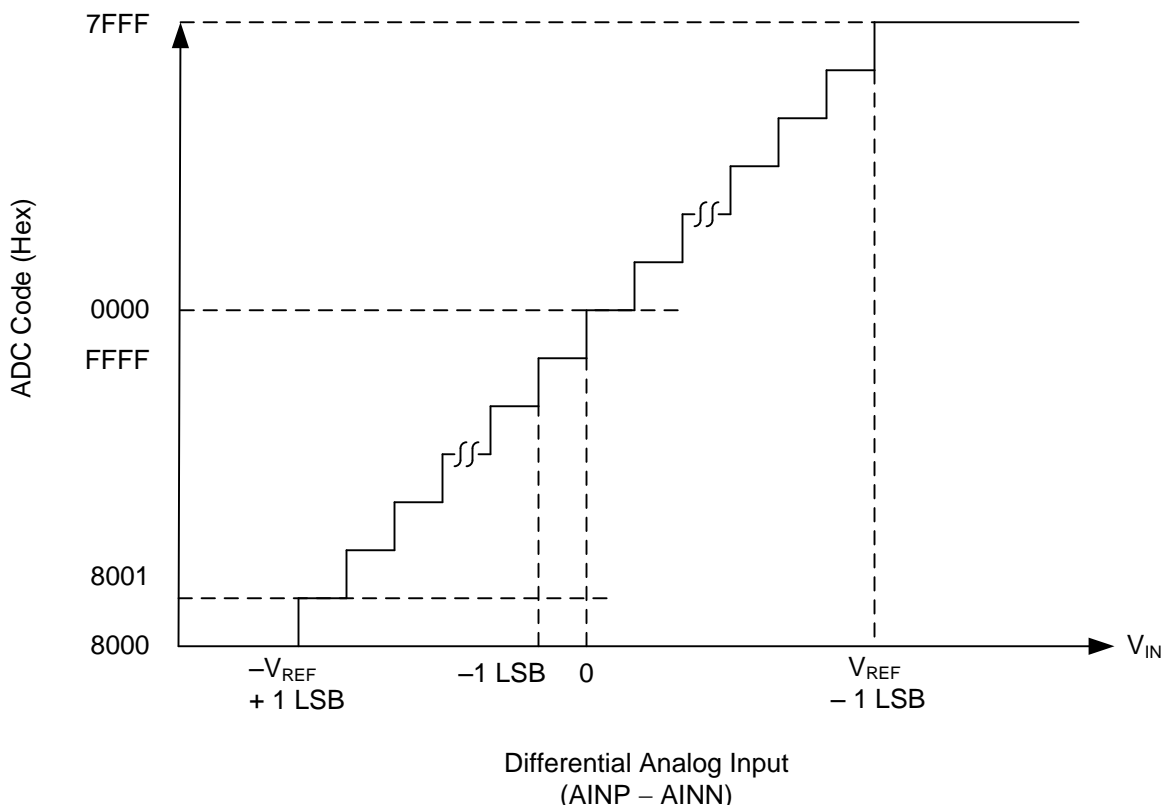
Figure 49. Transfer Characteristics
