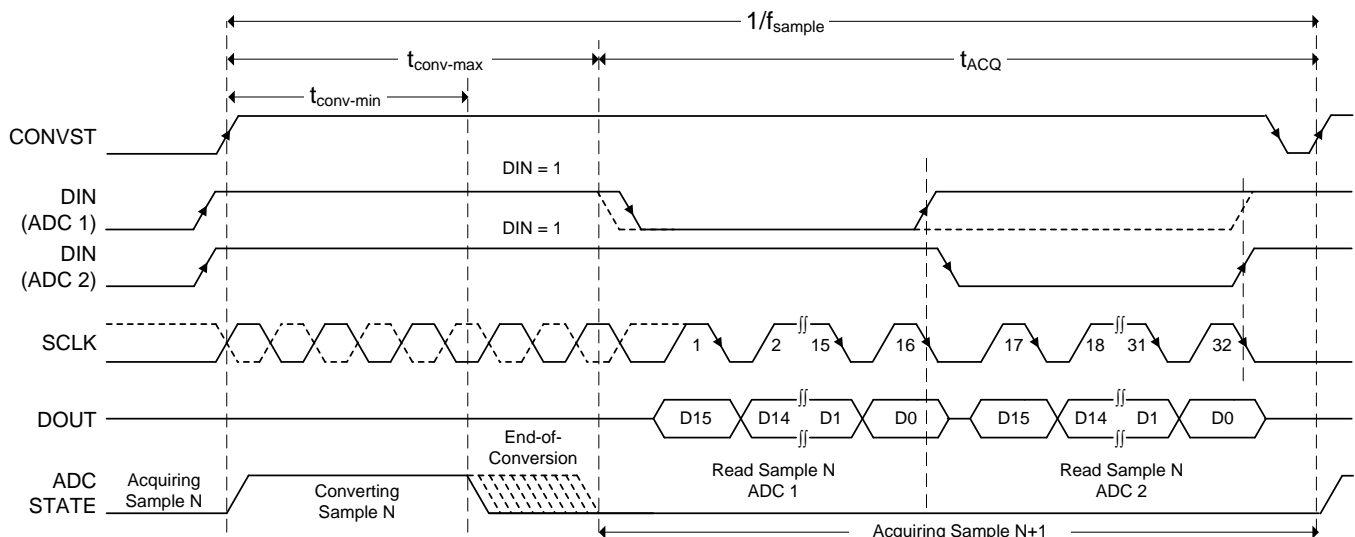
Figure 57. Interface Timing Diagram: Two ADCs with 4-Wire \overline{CS} Mode Without a Busy Indicator
