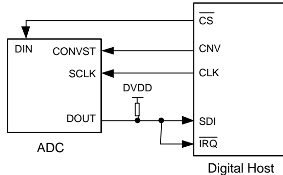
Figure 58. Connection Diagram: 4-Wire \overline{\text{CS}} Mode With a Busy Indicator
