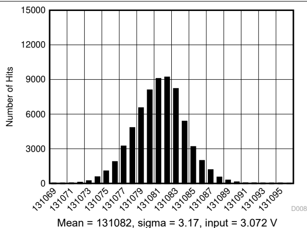
FIG 6-20. DC Histogram for Mid-Scale Inputs (0 V–6.144 V)
