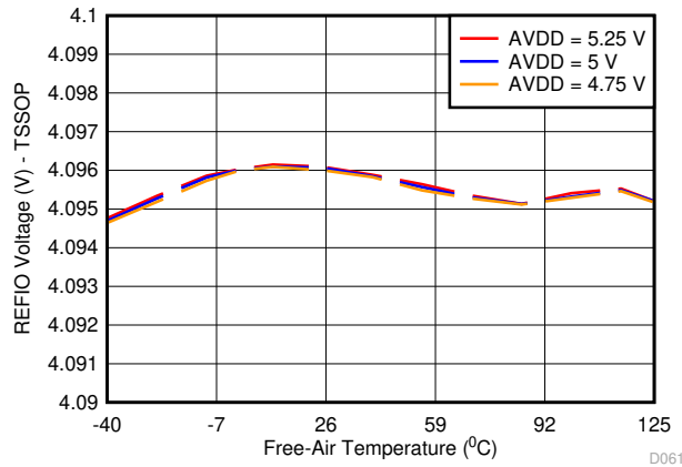
Figure 7-10. REFIO Voltage Variation Across AVDD and Temperature
