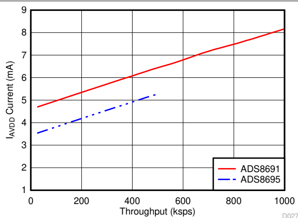
FIG 6-43. AVDD Current vs Throughput
