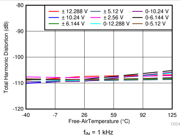
FIG 6-41. THD vs Temperature
