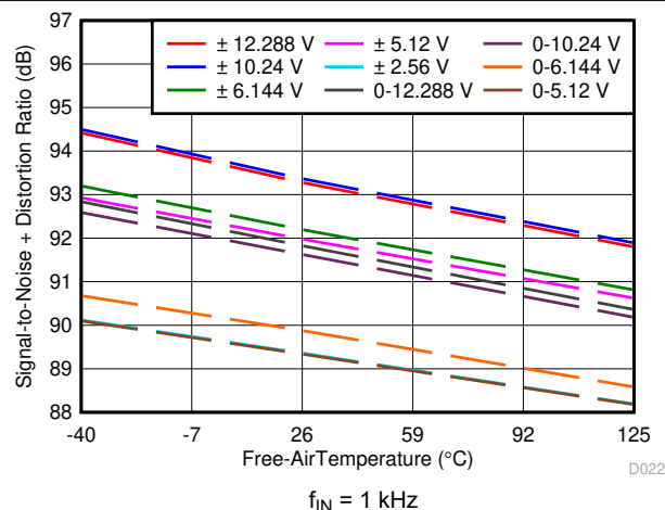
FIG 6-39. SINAD vs Temperature
