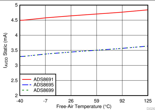
FIG 6-42. AVDD Current vs Temperature
