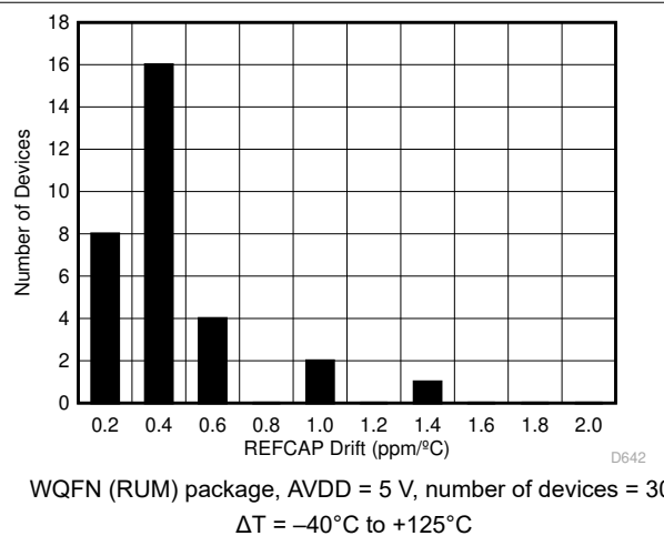
Figure 7-18. Reference Buffer Temperature Drift Histogram (RUM Package)
