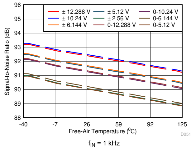
Figure 6-37. SNR vs Temperature
