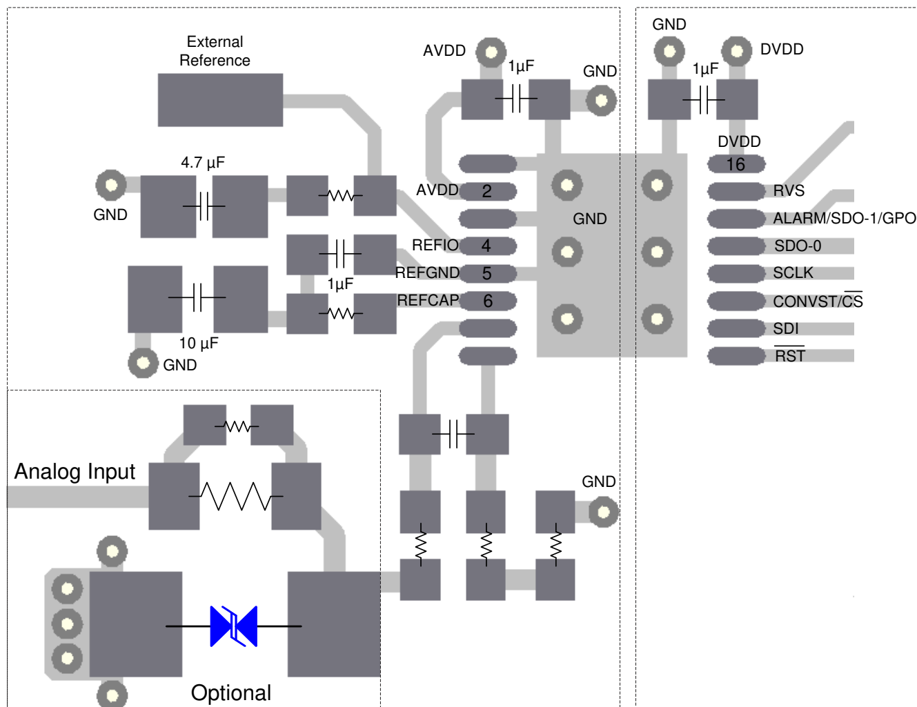
8-12. Board Layout for the ADS868x
