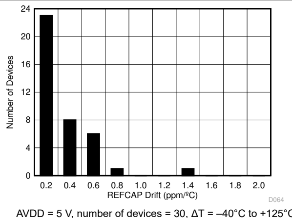
Figure 7-16. Reference Buffer Temperature Drift Histogram (PW Package)
