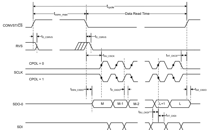
Figure 6-3. Standard SPI Interface Timing Diagram for CPHA = 0
