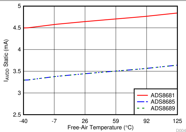
6-42. AVDD Current vs Temperature
