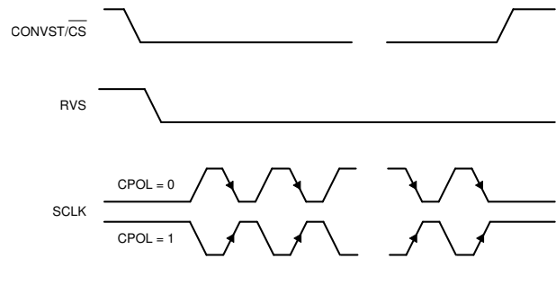
图 7-29. Standard SPI Timing Protocol (CPHA = 1, Single SDO-x)
