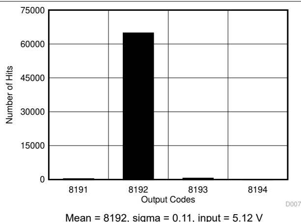
FIG 6-19. DC Histogram for Mid-Scale Inputs (0 V–10.24 V)
