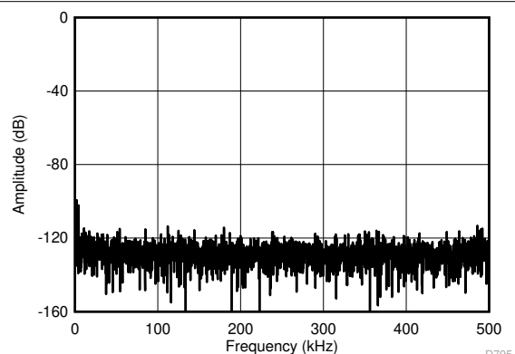
FIG 8-4. FFT Plot With an AC Common-Mode at 1 MSPS
