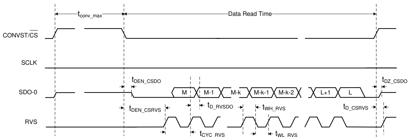
6-8. multiSPI Source-Synchronous Internal Clock Serial Interface Timing Diagram
