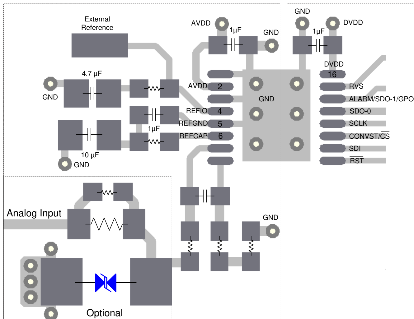
✎ 10-1. Board Layout for the ADS867x
