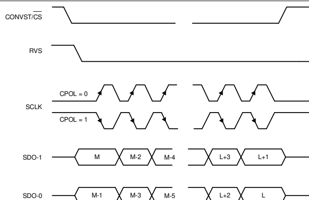
图 7-30. Standard SPI Timing Protocol (CPHA = 0, Dual SDO-x)
