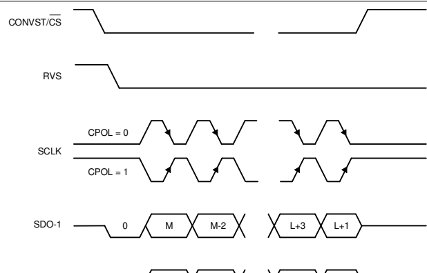
图 7-31. Standard SPI Timing Protocol (CPHA = 1, Dual SDO-x)
