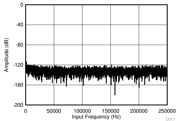
图 6-34. Typical FFT Plot (All Ranges) for the ADS8675
