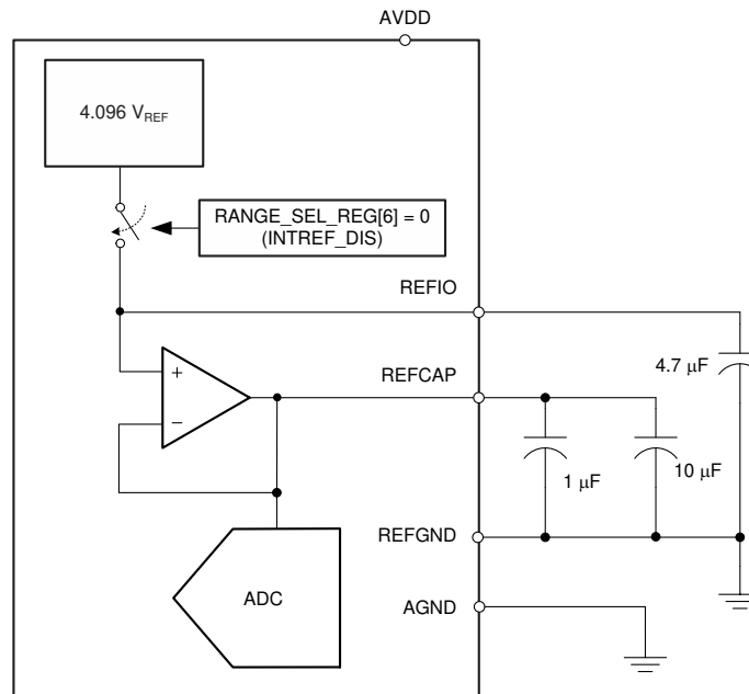
7-7. Device Connections for Using an Internal 4.096-V Reference
