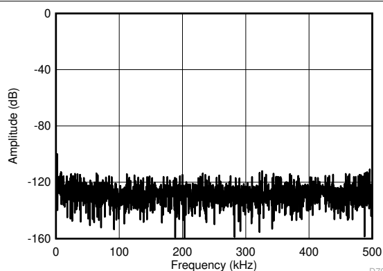
FIG 8-3. FFT Plot With a DC Common-Mode at 1 MSPS
