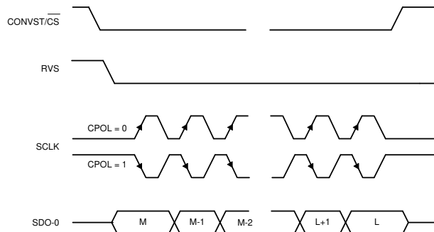
图 7-28. Standard SPI Timing Protocol (CPHA = 0, Single SDO-x)
