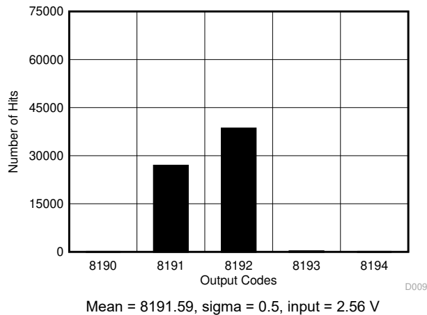
Figure 6-21. DC Histogram for Mid-Scale Inputs (0 V–5.12 V)
