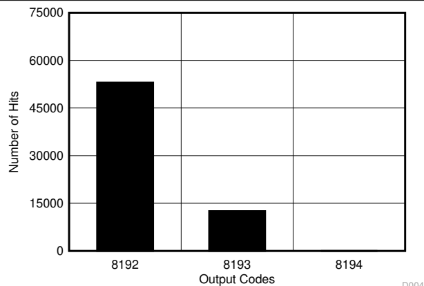
FIG 6-16. DC Histogram for Mid-Scale Inputs ( \pm 5.12\text{ V} )
