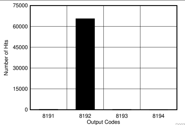
FIG 6-15. DC Histogram for Mid-Scale Inputs ( \pm 6.144\text{ V} )
