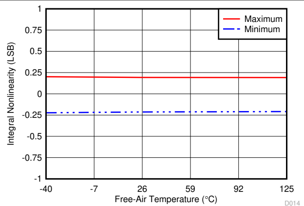
FIG 6-24. Typical INL for All Codes (All Bipolar Ranges)
