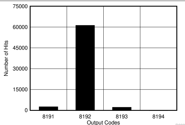
FIG 6-18. DC Histogram for Mid-Scale Inputs (0 V–12.288 V)
