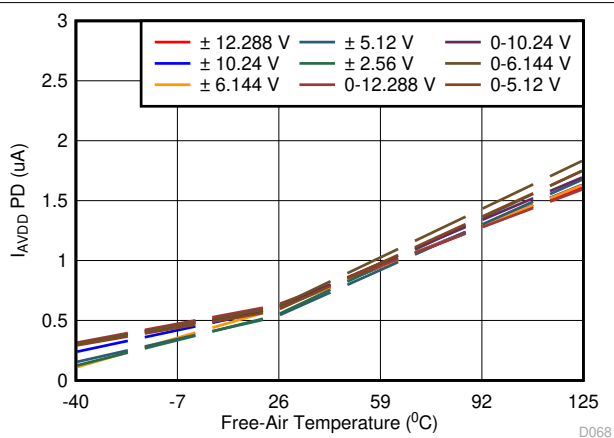
FIG 6-45. AVDD Current vs Temperature (Power-Down Mode)
