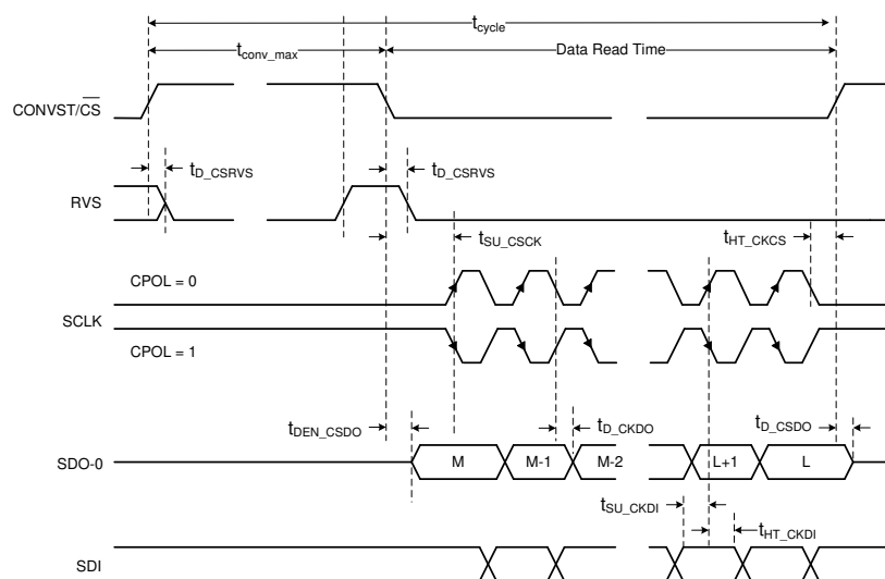
Figure 6-3. Standard SPI Interface Timing Diagram for \text{CPHA} = 0
