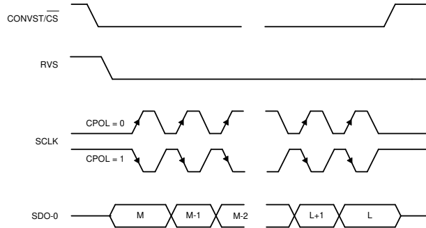
図 7-28. Standard SPI Timing Protocol (CPHA = 0, Single SDO-x)
