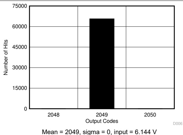
FIG 6-18. DC Histogram for Mid-Scale Inputs ( 0\text{ V} – 12.288\text{ V} )
