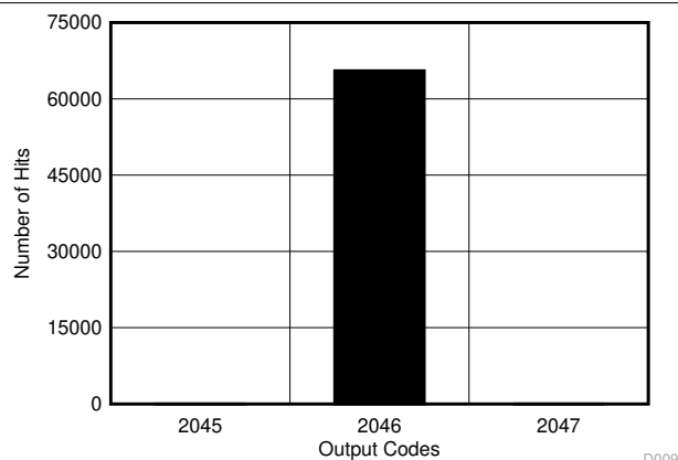
FIG 6-21. DC Histogram for Mid-Scale Inputs (0 V–5.12 V)
