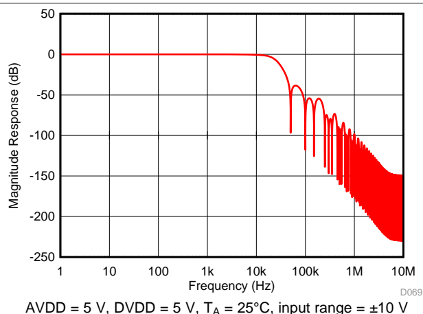
Figure 79. Digital Filter Response for OSR = 4
