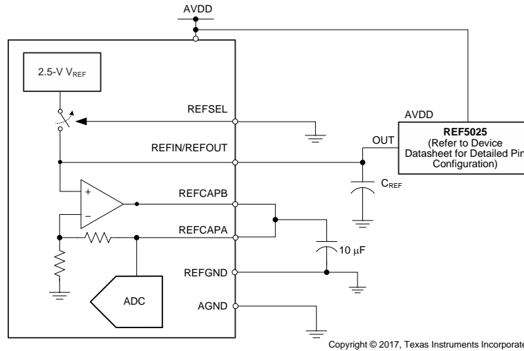
✎ 61. Device Connections for Using an External 2.5-V Reference
