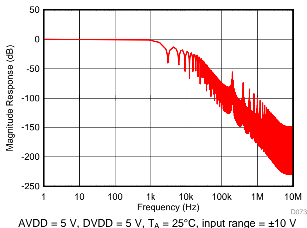
Figure 83. Digital Filter Response for OSR = 64
