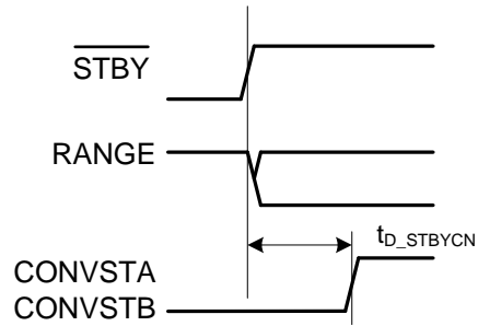
図 8. Exit Standby Mode Timing Diagram
