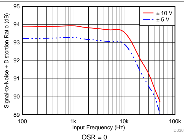
FIG 40. SINAD vs Input Frequency for Different Input Ranges
