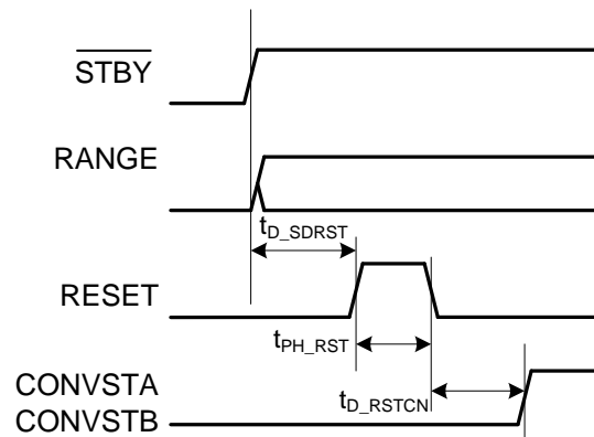
図 9. Exit Shutdown Mode Timing Diagram
