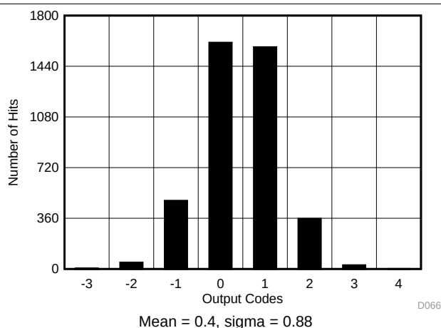
76. DC Histogram for OSR32
