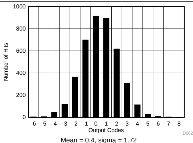
72. DC Histogram for OSR2
