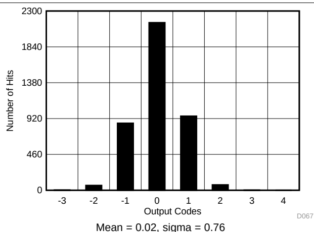
77. DC Histogram for OSR64
