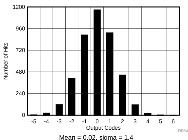
74. DC Histogram for OSR8
