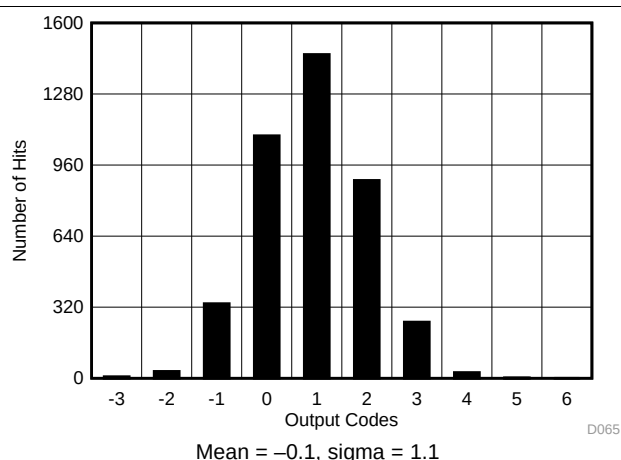
75. DC Histogram for OSR16
