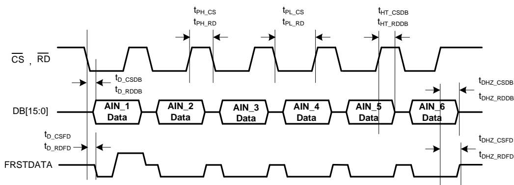
Figure 3. Parallel Data Read Operation, \overline{CS} and \overline{RD} Tied Together
