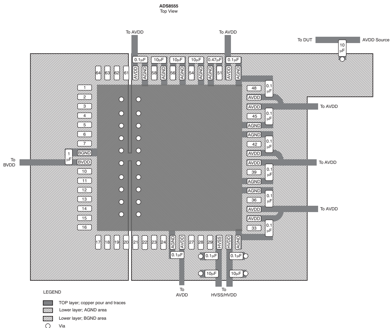
Figure 40. Layout Recommendation
