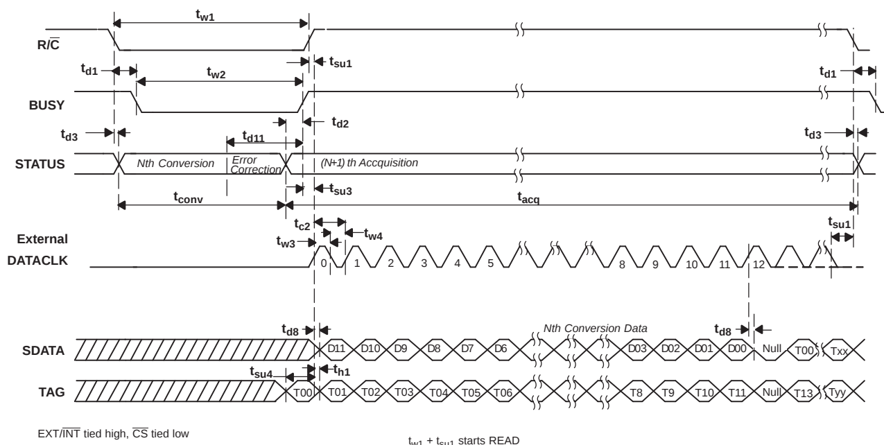
Figure 38. Read After Conversion (Discontinuous External \overline{DATACLK} )
