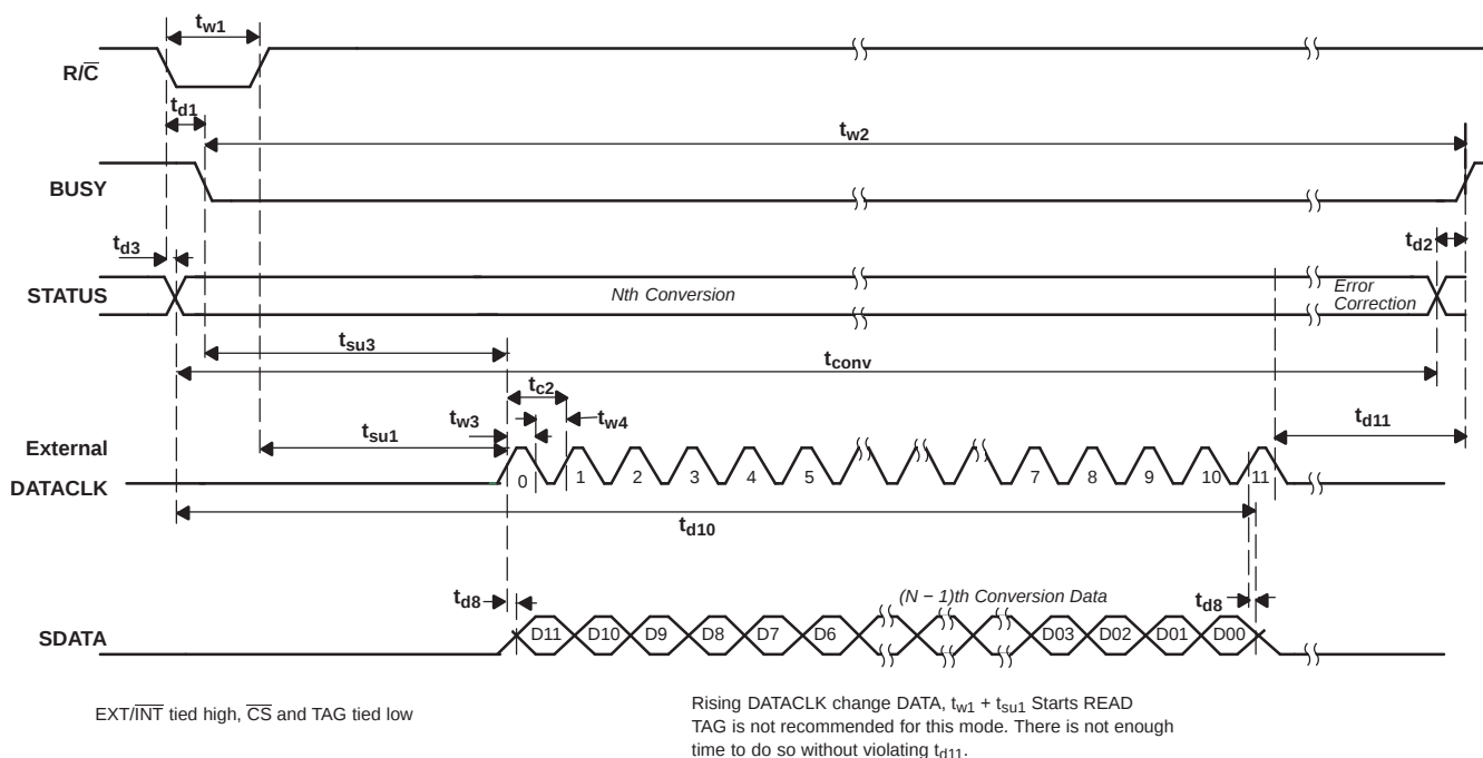
Figure 39. Read During Conversion (Discontinuous External \overline{DATACLK} )
