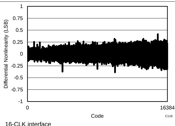
Figure 44. Typical DNL
