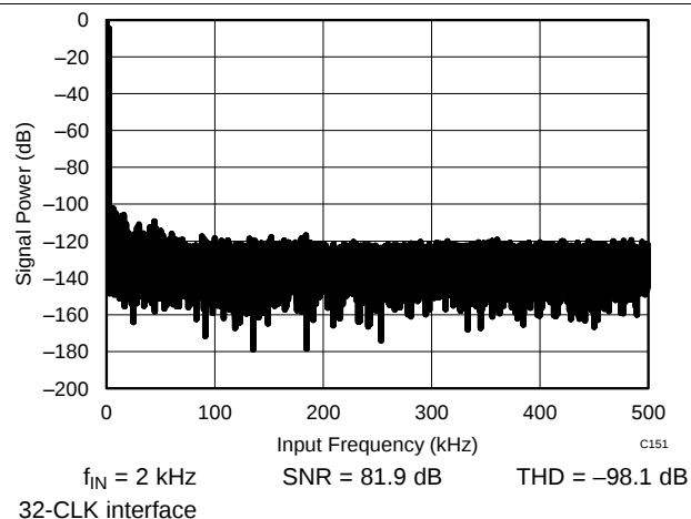
Figure 26. Typical FFT
