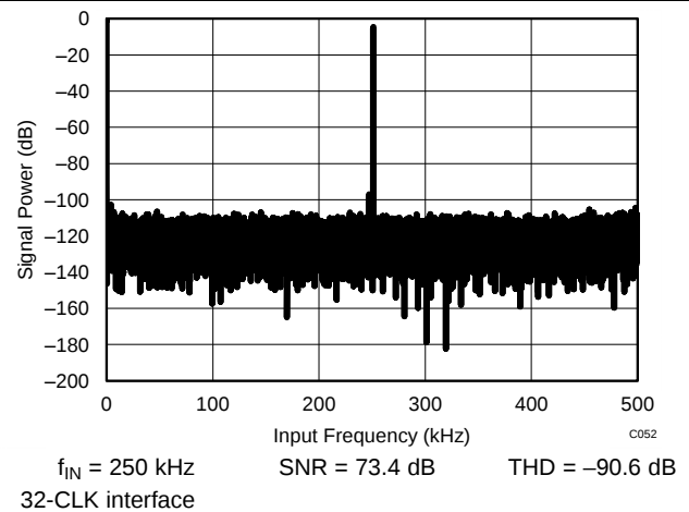
Figure 55. Typical FFT
