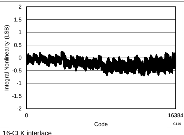
Figure 45. Typical INL
