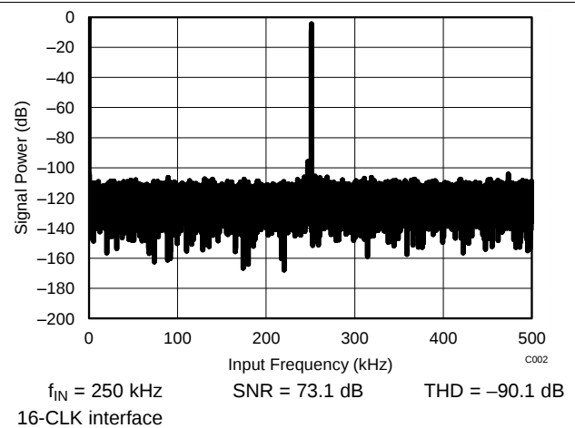
Figure 53. Typical FFT
