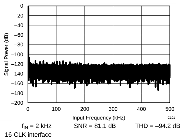
Figure 24. Typical FFT
