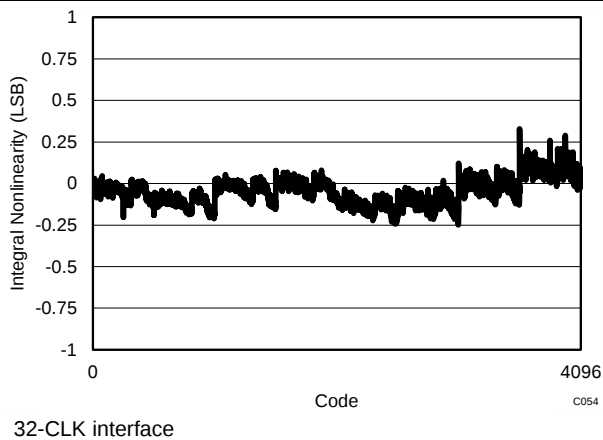
Figure 75. Typical INL
