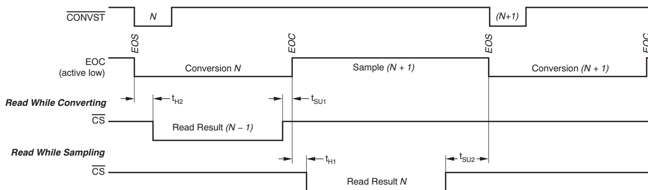
Figure 43. Read While Converting vs Read While Sampling (Manual-Trigger Mode)
