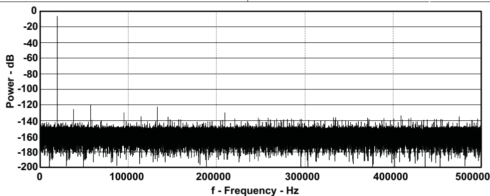
Figure 68. TYPICAL FFT
